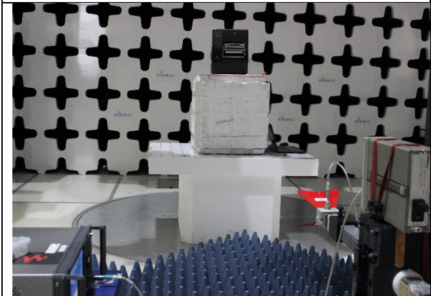
Radiated Emissions (>1GHz) – Front View
