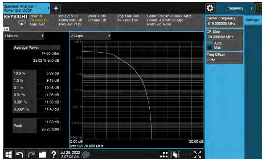
Band26-CH26740-819MHz-3MHz Bandwidth-QPSK
