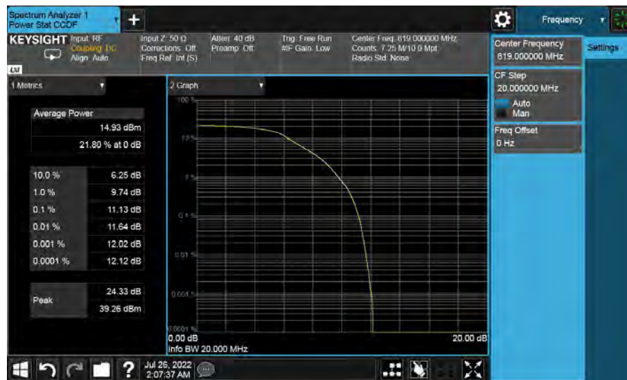
Band26-CH26740-819MHz-5MHz Bandwidth-QPSK
