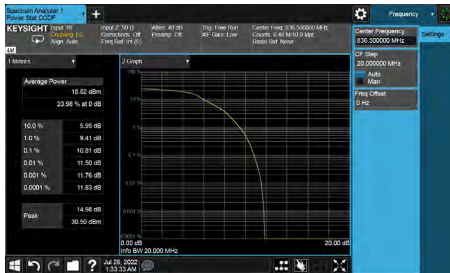
Band26-CH26915-836.5MHz-10MHz Bandwidth-QPSK
