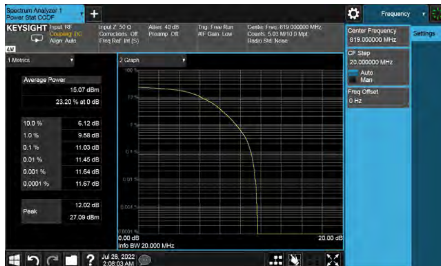
Band26-CH26740-819MHz-5MHz Bandwidth-16QAM
