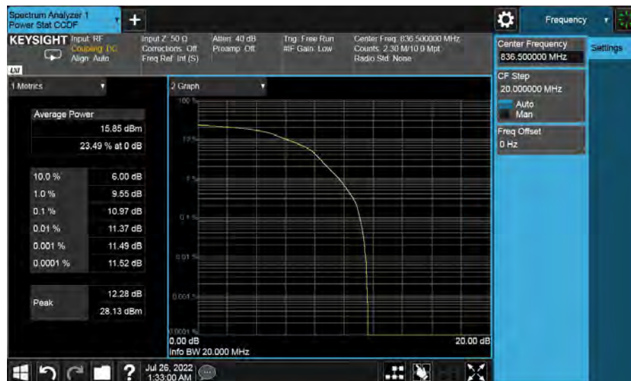
Band26-CH26915-836.5MHz-10MHz Bandwidth-16QAM
