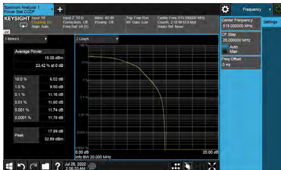
Band26-CH26740-819MHz-3MHz Bandwidth-16QAM
