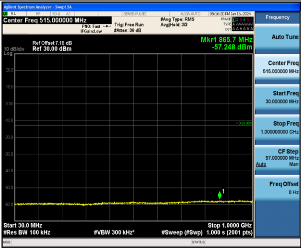
Band4_1.4MHz_16QAM_20175_1RB#0_30~1000_30~1000
