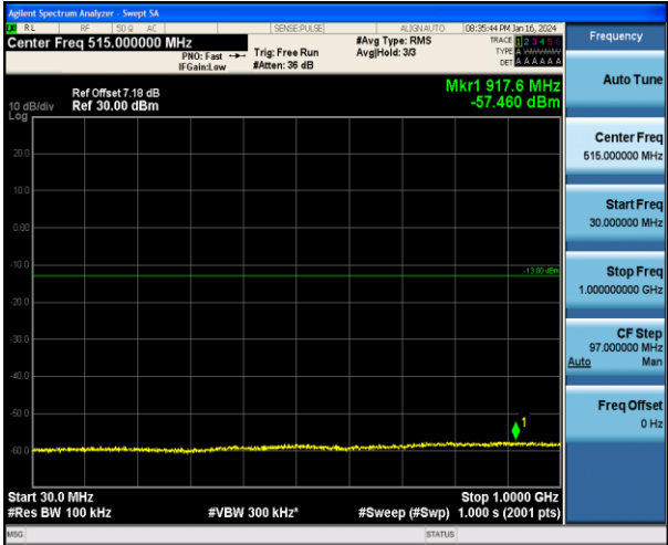
Band4_3MHz_QPSK_20385_1RB#0_30~1000_30~1000
