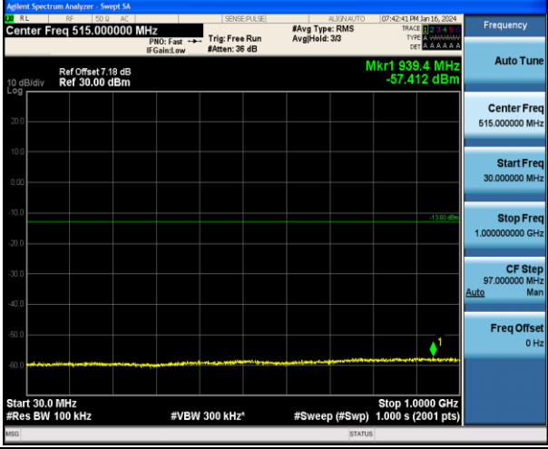
Band2_15MHz_16QAM_18675_1RB#0_30~1000_30~1000
