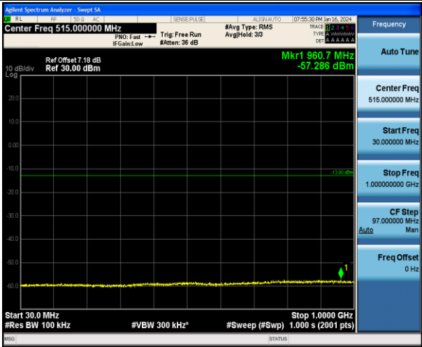
Band2_20MHz_QPSK_18700_1RB#0_30~1000_30~1000
