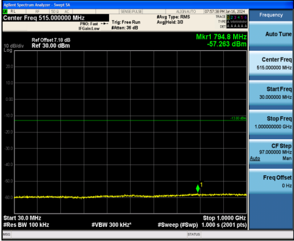
Band2_20MHz_QPSK_19100_1RB#0_30~1000_30~1000
