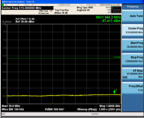
Band4_5MHz_QPSK_20375_1RB#0_30~1000_30~1000
