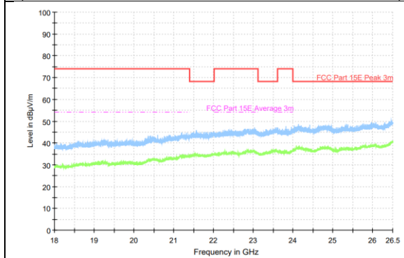
Radiated Spurious Emission (802.11ac 20M-MIMO, ch100, 18GHz-26.5GHz)
