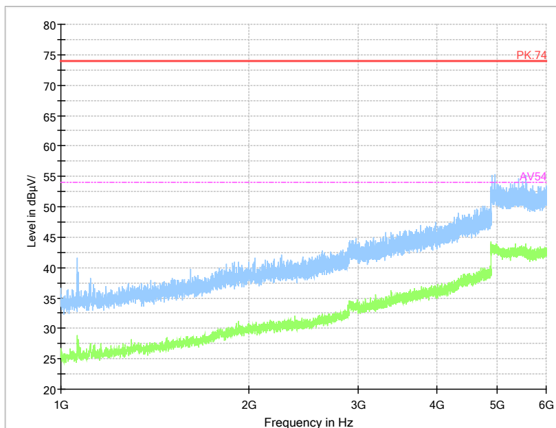
Pic9. Radiated emission (1GHz –6GHz)
