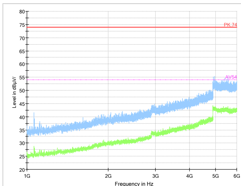
Pic18. Radiated emission (1GHz –6GHz)
