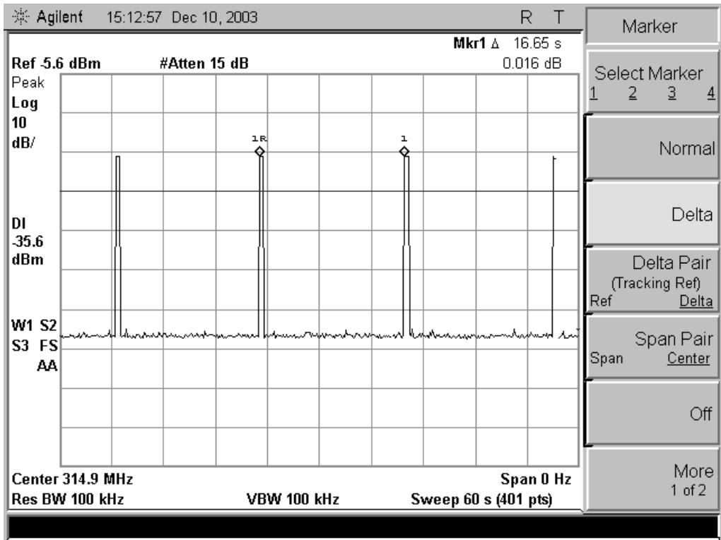
Figure 4. Transmission interval
