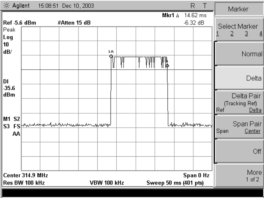
Figure 1. normal transmission
