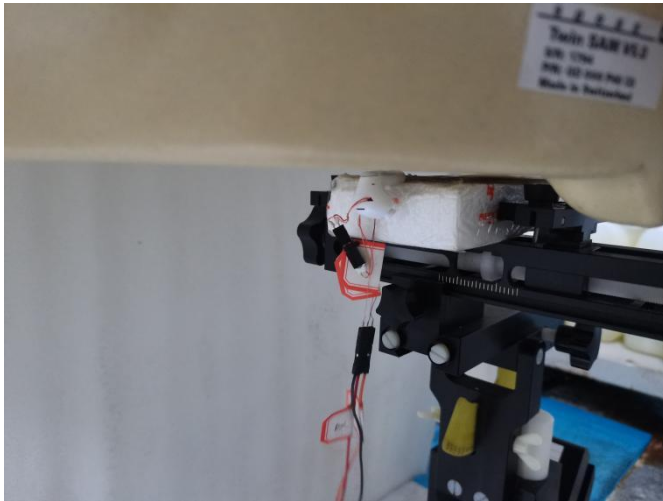
Fig-4.1 Rear Side of EUT with 0 cm Gap (Body Mode)
