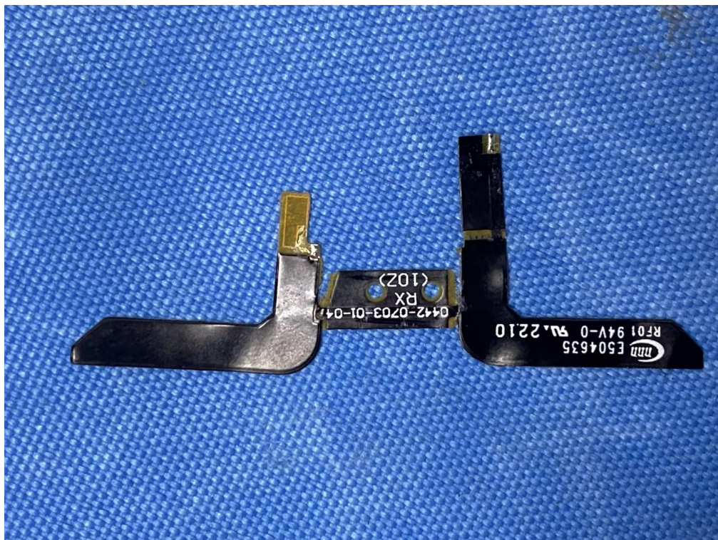
INTERNAL VIEW OF EUT (FIGURE 4)---Antenna 2
