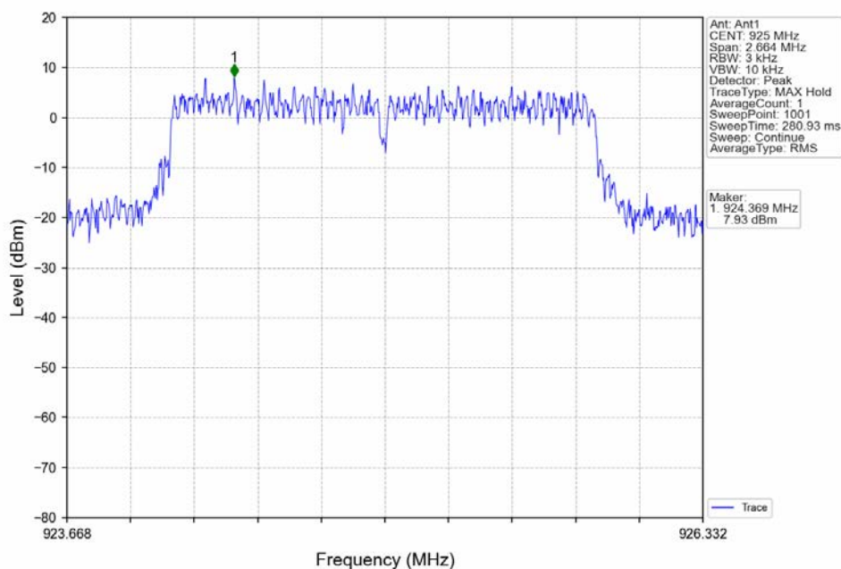
2M_HCH_925MHz_Ant1_NTNV
