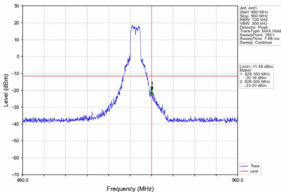
4M_HCH_922MHz_Ant1_NTNV
