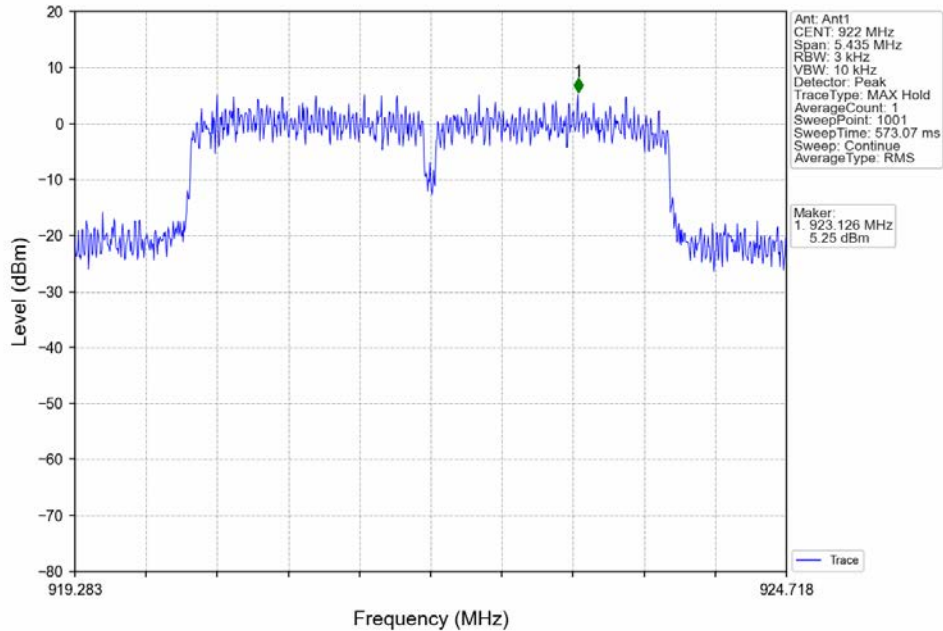
4M_HCH_922MHz_Ant1_NTNV
