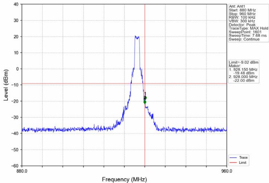
2M_HCH_925MHz_Ant1_NTNV
