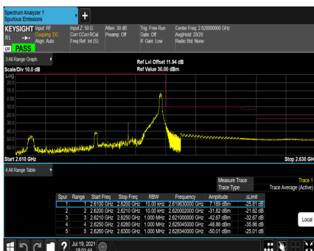
Band38-5MHz-16QAM-38225-1RB#24
