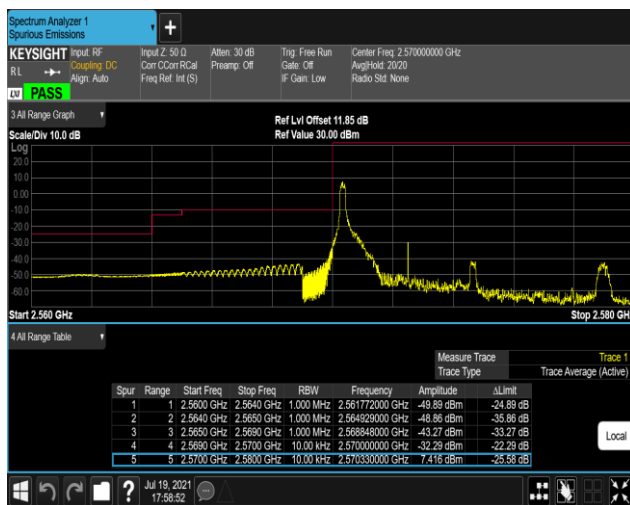
Band38-5MHz-16QAM-37775-25RB#0
