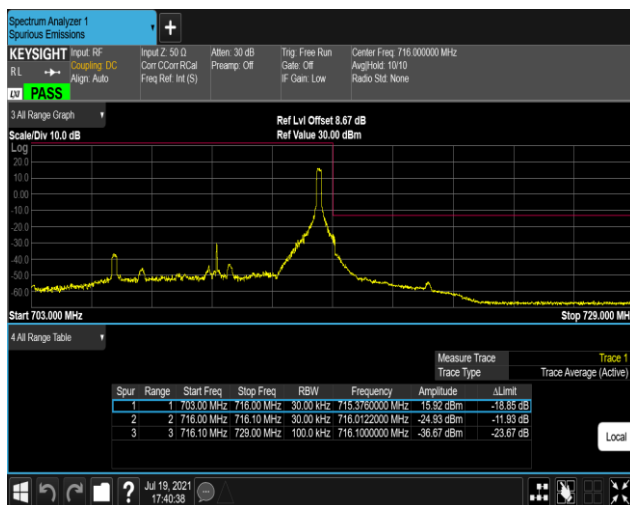
Band17-10MHz-QPSK-23800-1RB#49
