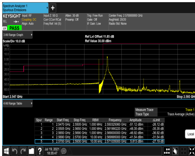
Band38-20MHz-QPSK-37850-100RB#0
