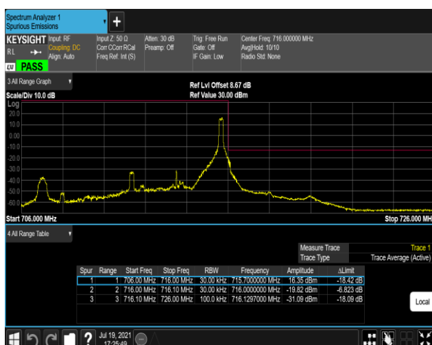
Band17-5MHz-QPSK-23825-1RB#24
