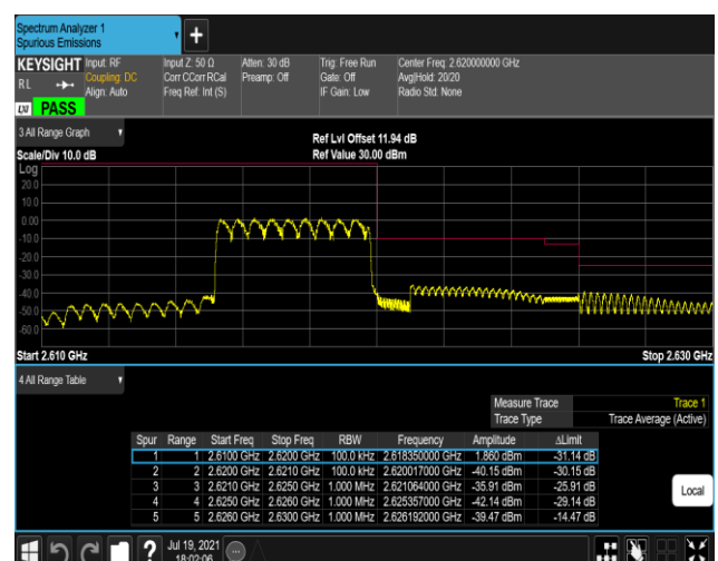
Band38-5MHz-QPSK-38225-25RB#0
