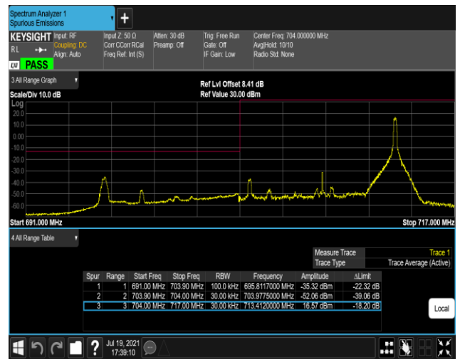
Band17-10MHz-QPSK-23800-1RB#0
