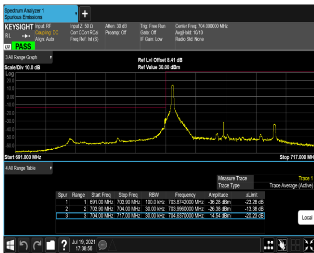
Band17-10MHz-16QAM-23780-50RB#0
