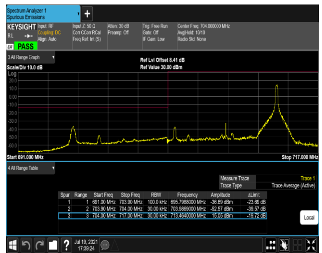
Band17-10MHz-16QAM-23800-1RB#0
