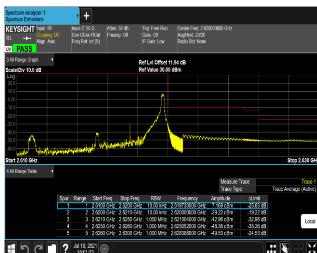
Band38-5MHz-QPSK-38225-1RB#24
