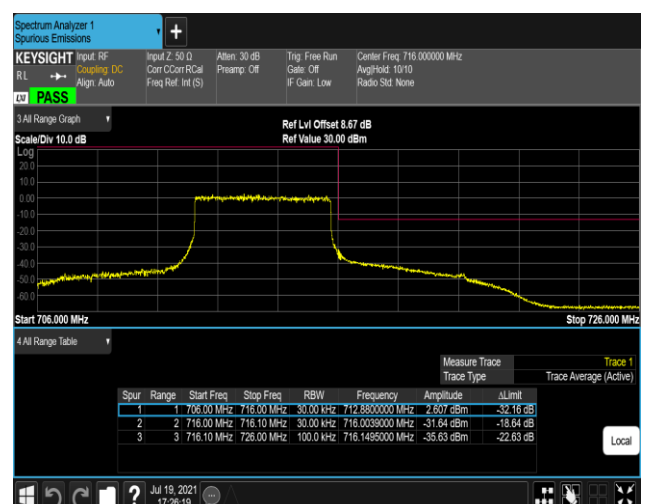
Band17-5MHz-QPSK-23825-25RB#0
