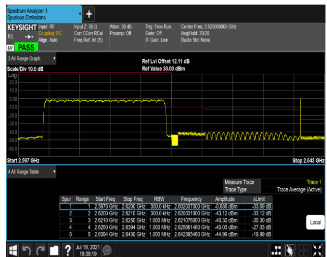
Band38-20MHz-QPSK-38150-100RB#0
