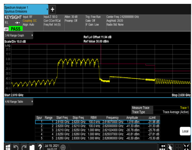
Band38-5MHz-16QAM-38225-25RB#0
