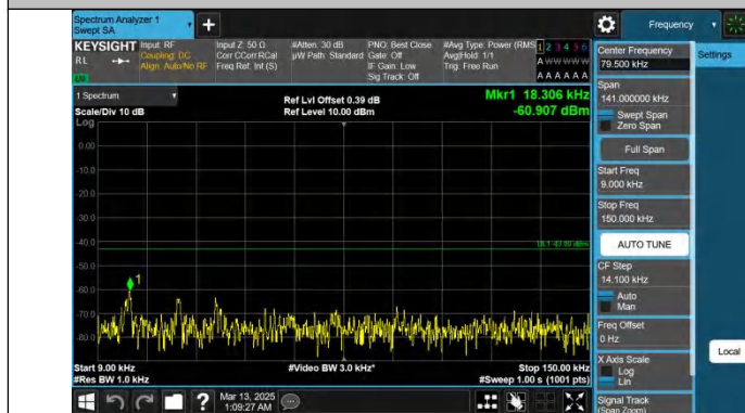
Band25-10MHz-QPSK-26090-1RB#0-0.009~0.15-PASS
