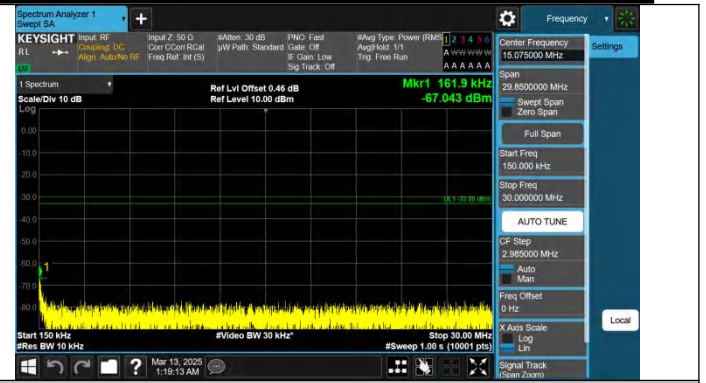
Band25-15MHz-QPSK-26115-1RB#0-0.15~30-PASS
