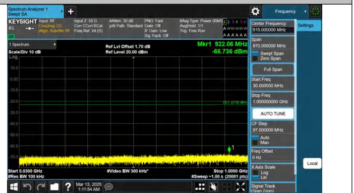
Band25-10MHz-QPSK-26365-1RB#49-30~1000-PASS
