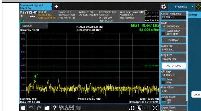
Band25-3MHz-QPSK-26675-1RB#0-0.009~0.15-PASS
