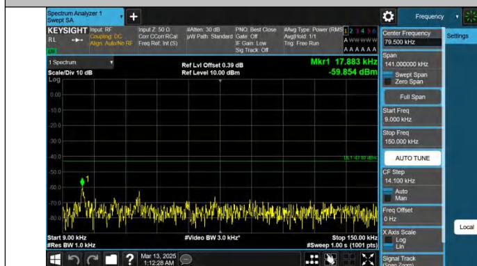
Band25-10MHz-QPSK-26640-1RB#0-0.009~0.15-PASS
