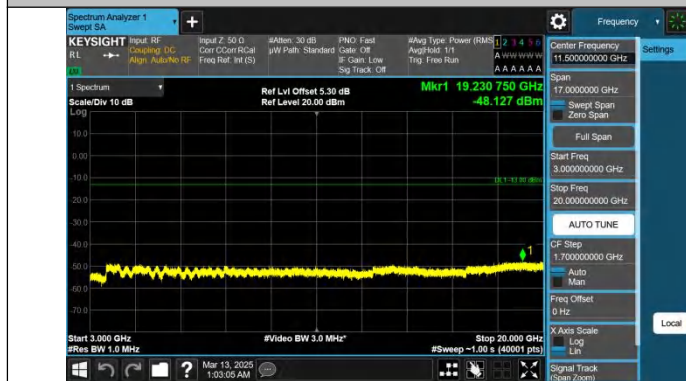
Band25-5MHz-QPSK-26665-1RB#0-3000~20000-PASS
