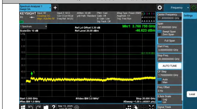
Band25-5MHz-QPSK-26365-1RB#0-3000~20000-PASS
