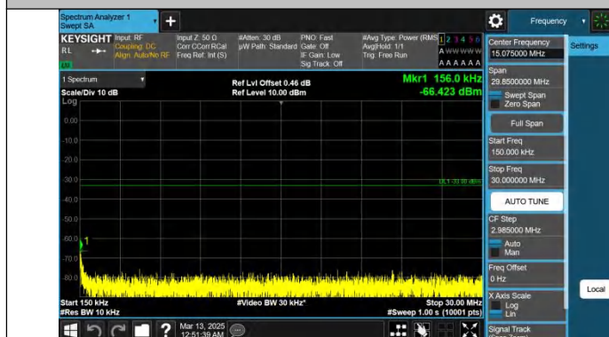
Band25-3MHz-QPSK-26365-1RB#14-0.15~30-PASS
