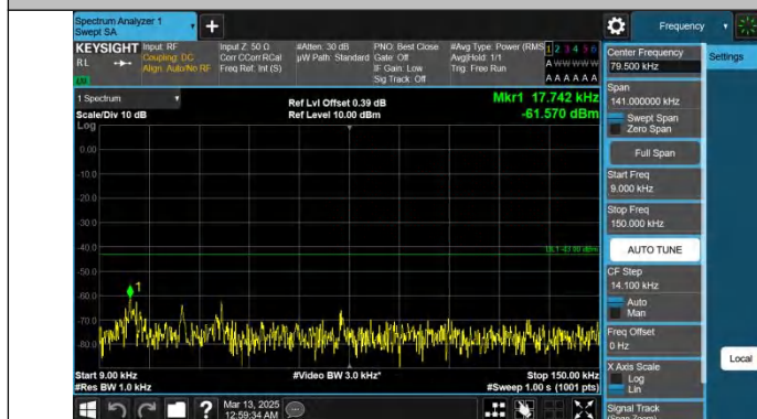
Band25-5MHz-QPSK-26065-1RB#0-0.009~0.15-PASS
