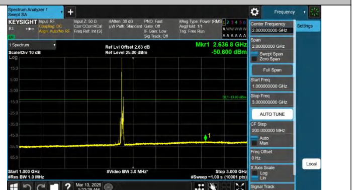
Band25-15MHz-QPSK-26615-1RB#0-1000~3000-PASS
