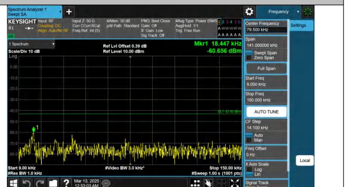
Band25-3MHz-QPSK-26675-1RB#14-0.009~0.15-PASS
