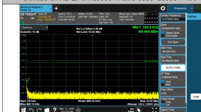
Band25-5MHz-QPSK-26365-1RB#24-0.15~30-PASS
