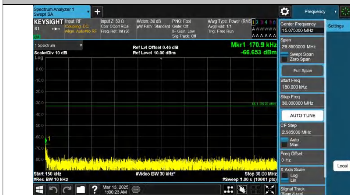
Band25-5MHz-QPSK-26065-1RB#24-0.15~30-PASS
