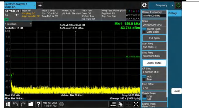
Band25-5MHz-QPSK-26665-1RB#0-0.15~30-PASS
