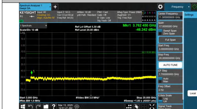
Band25-3MHz-QPSK-26365-1RB#0-3000~20000-PASS
