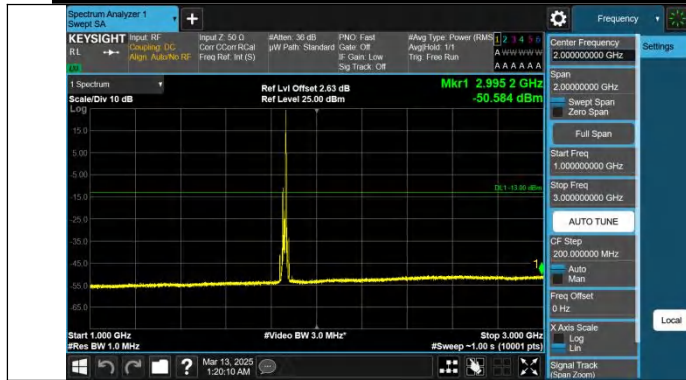
Band25-15MHz-QPSK-26115-1RB#74-1000~3000-PASS
