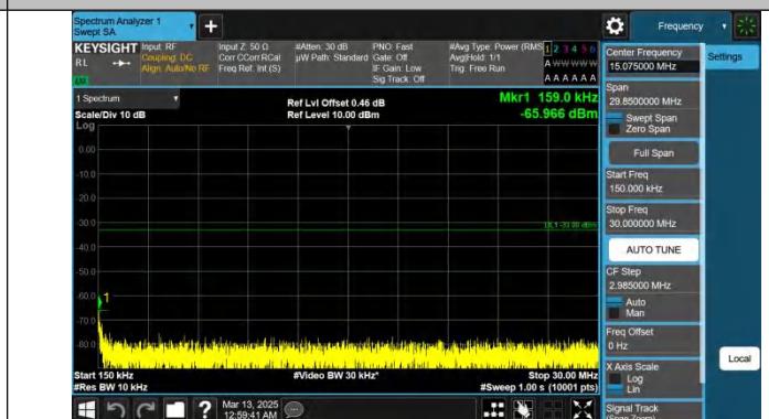
Band25-5MHz-QPSK-26065-1RB#0-0.15~30-PASS
