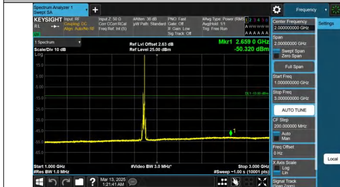
Band25-15MHz-QPSK-26365-1RB#74-1000~3000-PASS
