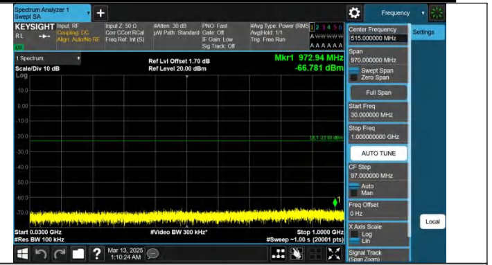
Band25-10MHz-QPSK-26090-1RB#49-30~1000-PASS
