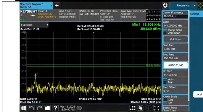
Band25-3MHz-QPSK-26365-1RB#0-0.009~0.15-PASS
