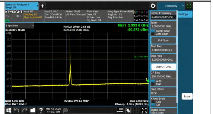
Band25-15MHz-QPSK-26115-1RB#0-1000~3000-PASS
