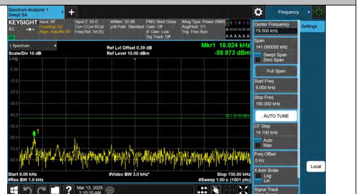
Band25-10MHz-QPSK-26090-1RB#49-0.009~0.15-PASS
