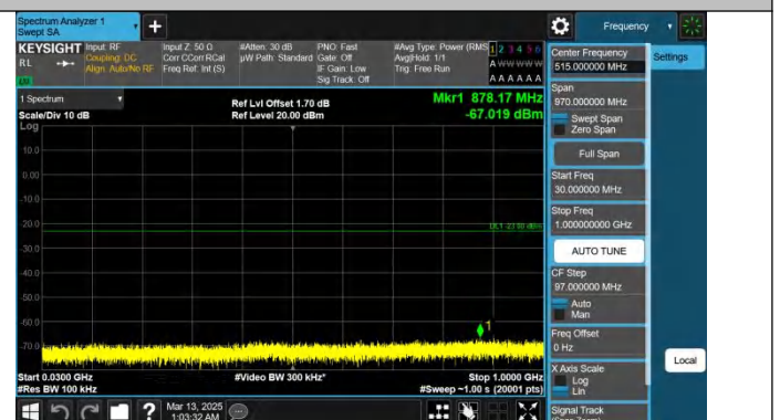
Band25-5MHz-QPSK-26665-1RB#24-30~1000-PASS
