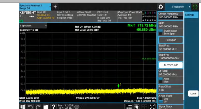
Band25-3MHz-QPSK-26365-1RB#14-30~1000-PASS
