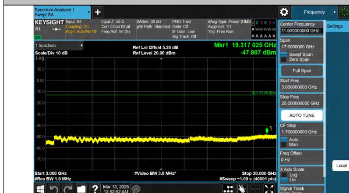
Band25-3MHz-QPSK-26675-1RB#0-3000~20000-PASS
