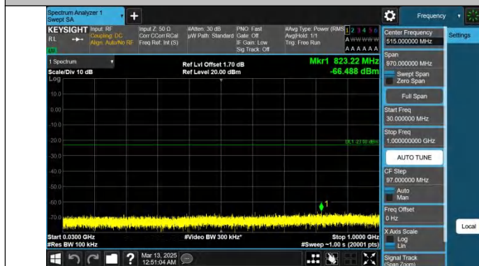
Band25-3MHz-QPSK-26365-1RB#0-30~1000-PASS
