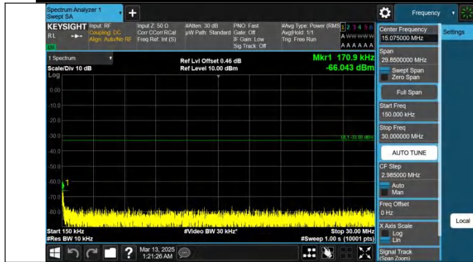
Band25-15MHz-QPSK-26365-1RB#74-0.15~30-PASS
