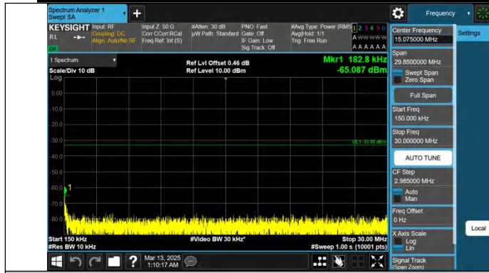
Band25-10MHz-QPSK-26090-1RB#49-0.15~30-PASS
