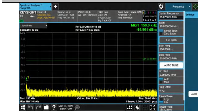
Band25-10MHz-QPSK-26365-1RB#49-0.15~30-PASS
