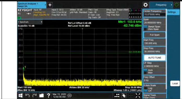
Band25-3MHz-QPSK-26365-1RB#0-0.15~30-PASS
