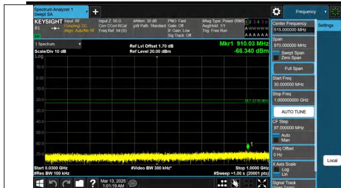
Band25-5MHz-QPSK-26365-1RB#0-30~1000-PASS
