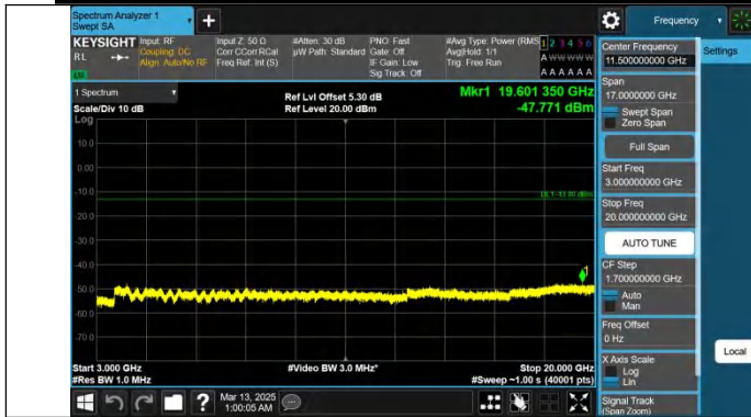
Band25-5MHz-QPSK-26065-1RB#0-3000~20000-PASS
