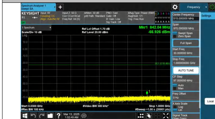
Band25-5MHz-QPSK-26665-1RB#0-30~1000-PASS
