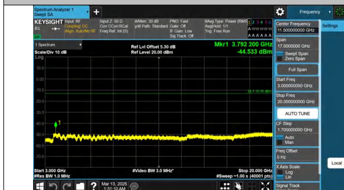
Band25-20MHz-QPSK-26590-1RB#0-3000~20000-PASS
