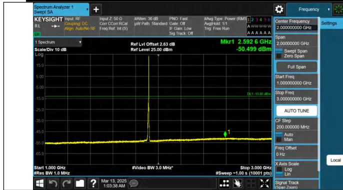
Band25-5MHz-QPSK-26665-1RB#24-1000~3000-PASS
