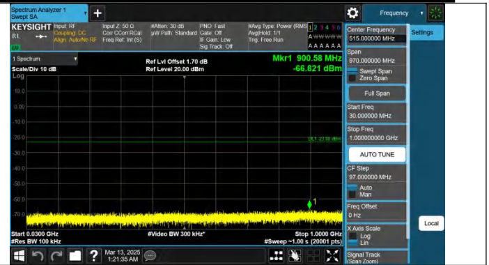
Band25-15MHz-QPSK-26365-1RB#74-30~1000-PASS
