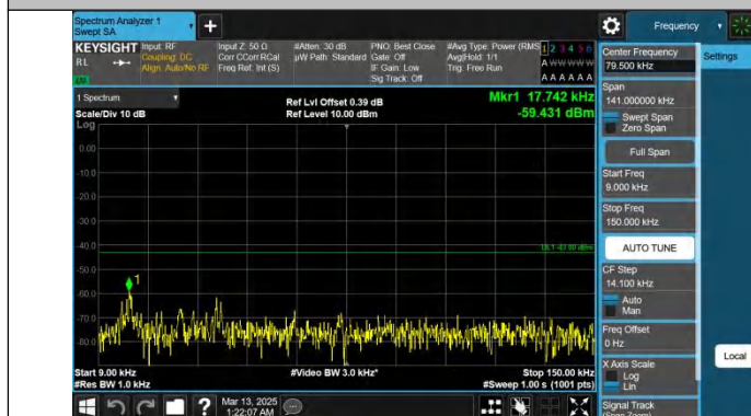
Band25-15MHz-QPSK-26615-1RB#0-0.009~0.15-PASS
