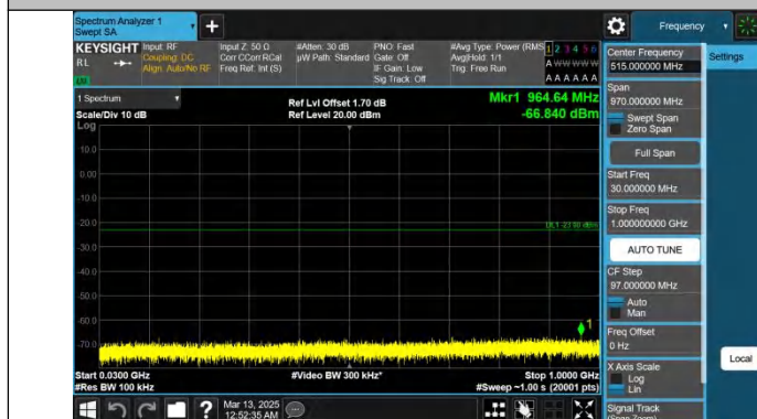
Band25-3MHz-QPSK-26675-1RB#0-30~1000-PASS
