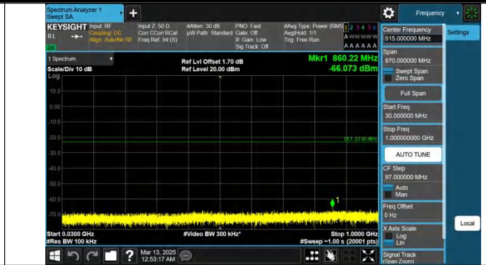
Band25-3MHz-QPSK-26675-1RB#14-30~1000-PASS
