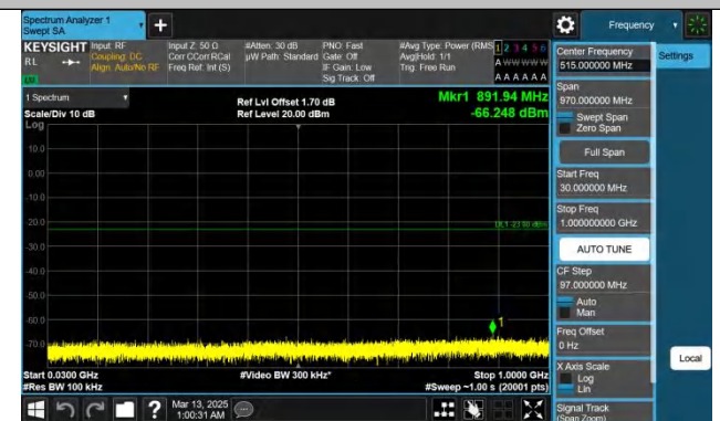
Band25-5MHz-QPSK-26065-1RB#24-30~1000-PASS
