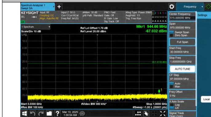
Band25-20MHz-QPSK-26590-1RB#0-30~1000-PASS
