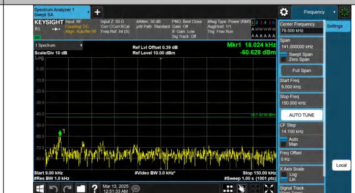
Band25-3MHz-QPSK-26365-1RB#14-0.009~0.15-PASS
