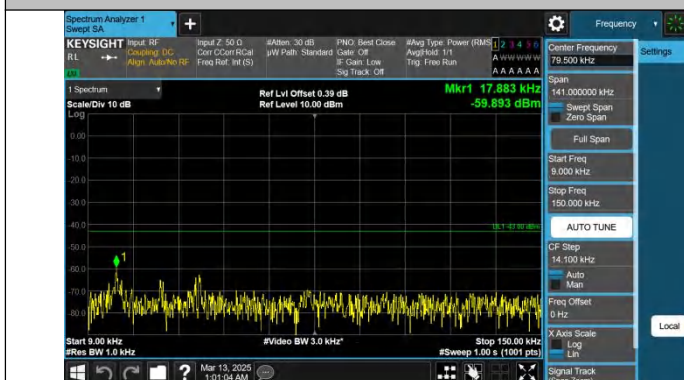
Band25-5MHz-QPSK-26365-1RB#0-0.009~0.15-PASS
