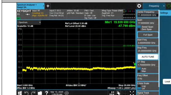
Band25-10MHz-QPSK-26090-1RB#0-3000~20000-PASS
