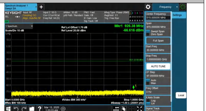
Band25-15MHz-QPSK-26115-1RB#74-30~1000-PASS
