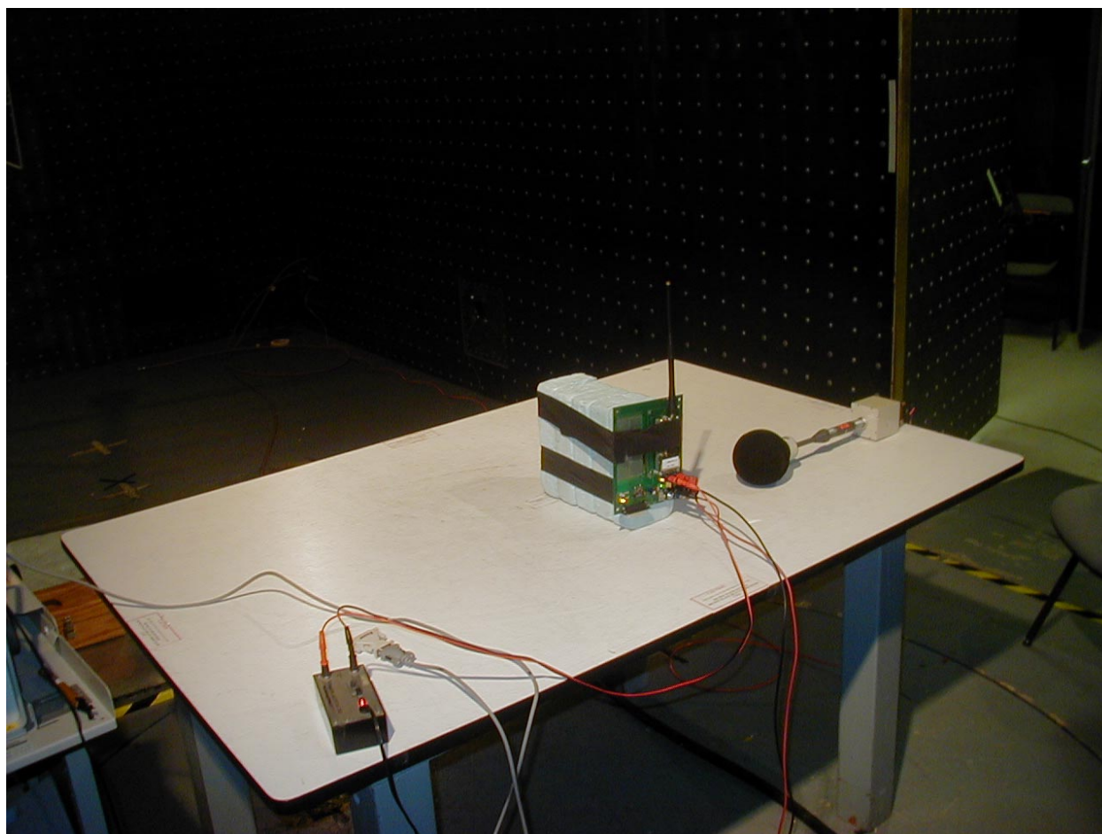
Setup Photo# 1
