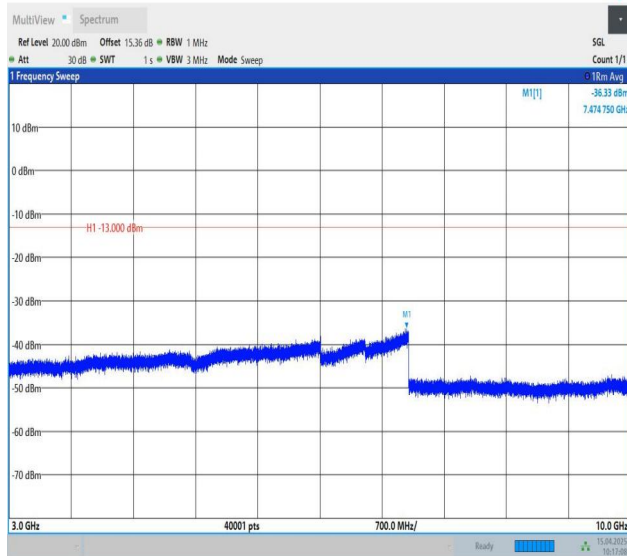
Band13-10MHz-QPSK-23230-1RB#0-3000~10000-PASS
