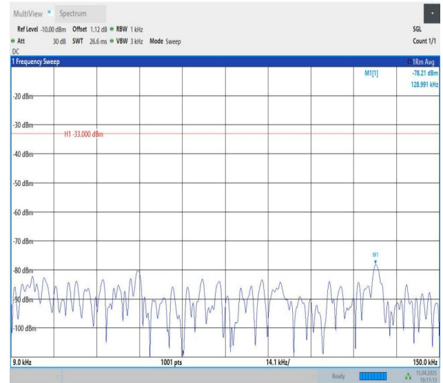
Band13-10MHz-QPSK-23230-1RB#49-0.009~0.15-PASS
