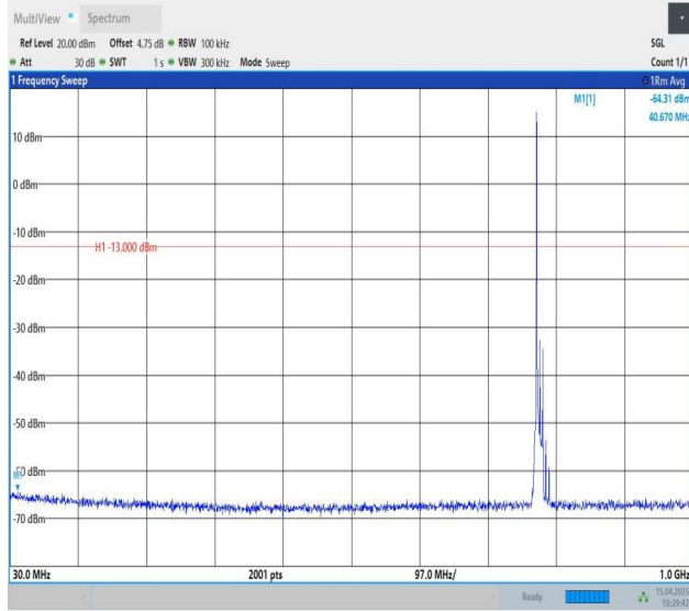
Band13-10MHz-QPSK-23230-1RB#0-30~1000-PASS
