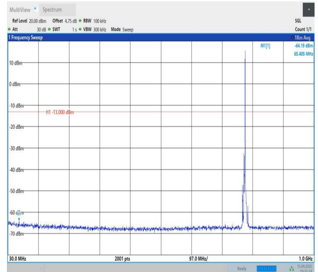
Band13-5MHz-QPSK-23205-1RB#24-30~1000-PASS
