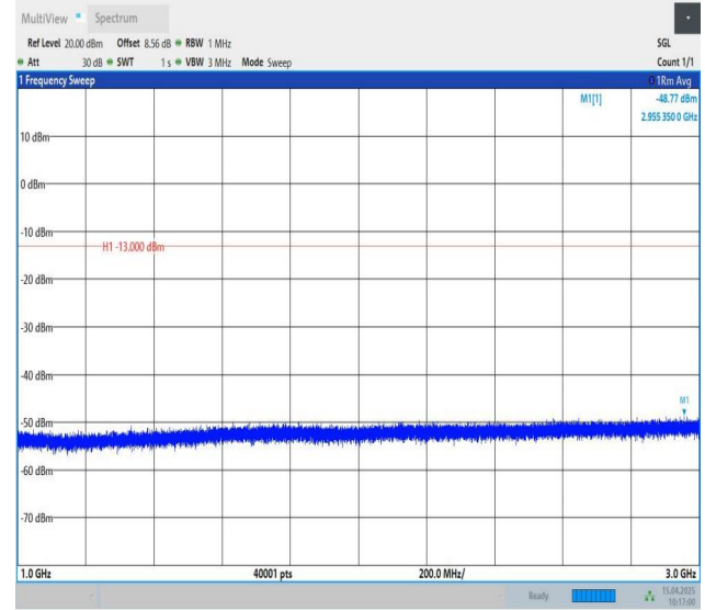
Band13-10MHz-QPSK-23230-1RB#0-1000~3000-PASS
