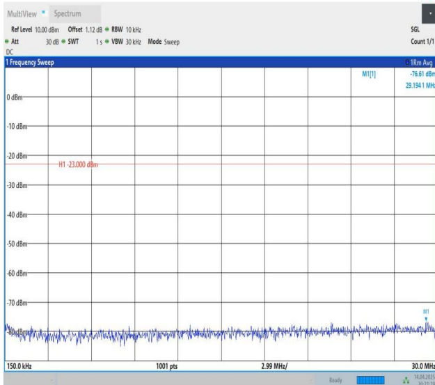
Band13-5MHz-QPSK-23205-1RB#24-0.15~30-PASS
