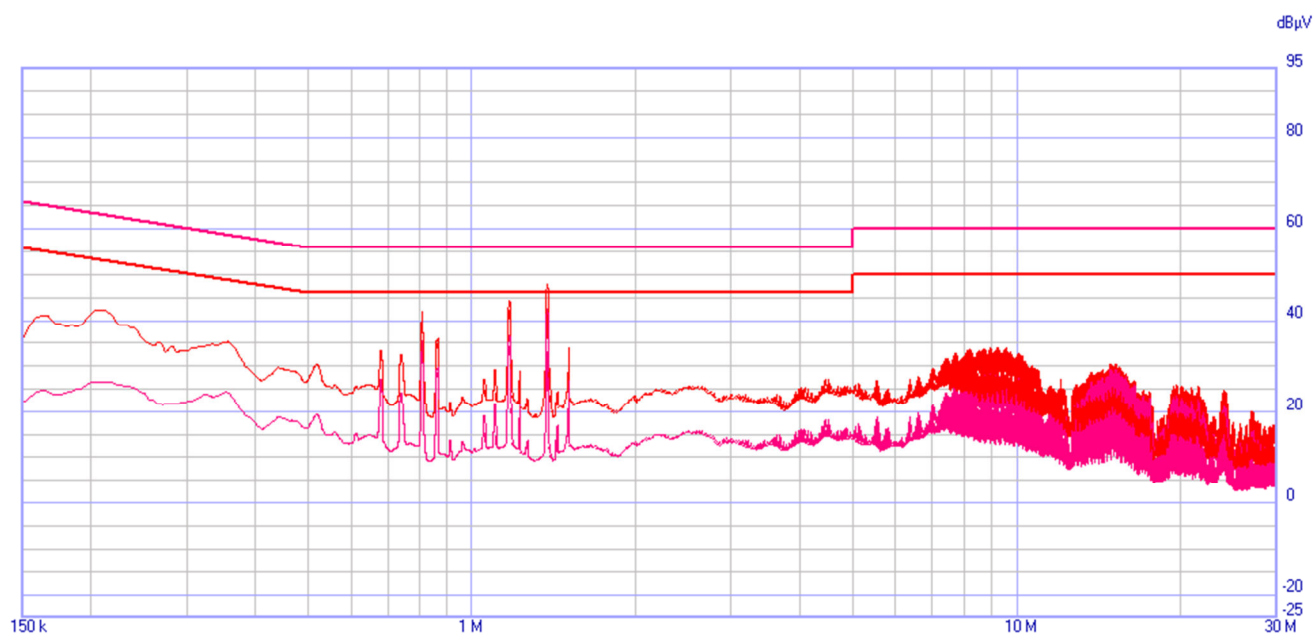
Plot 1: Conducted Emissions Limits, Line
