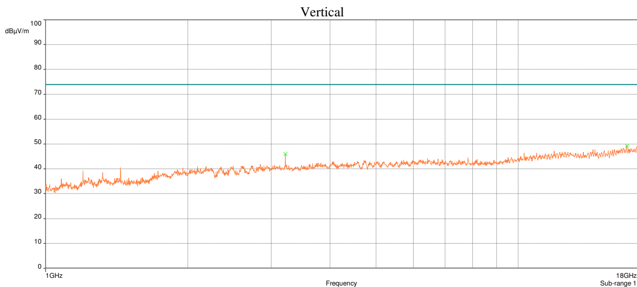
Plot 10: Radiated Spurious Emissions Requirements, 802.11g, Low Channel 2412MHz, Peak
