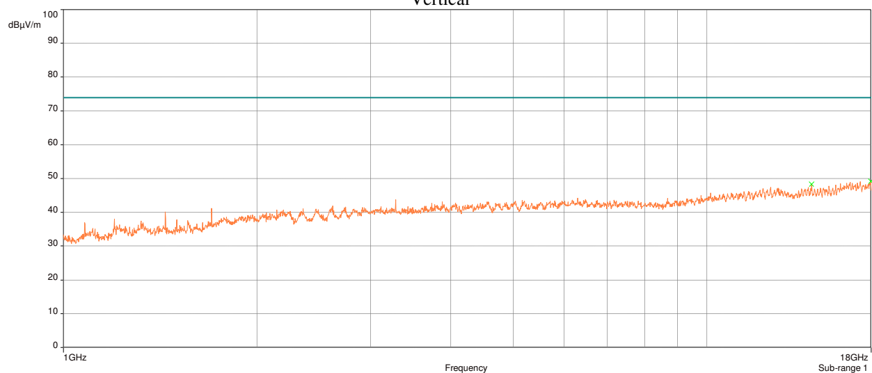
Plot 20: Radiated Spurious Emissions Requirements, 802.11n, High Channel 2462MHz, Peak
