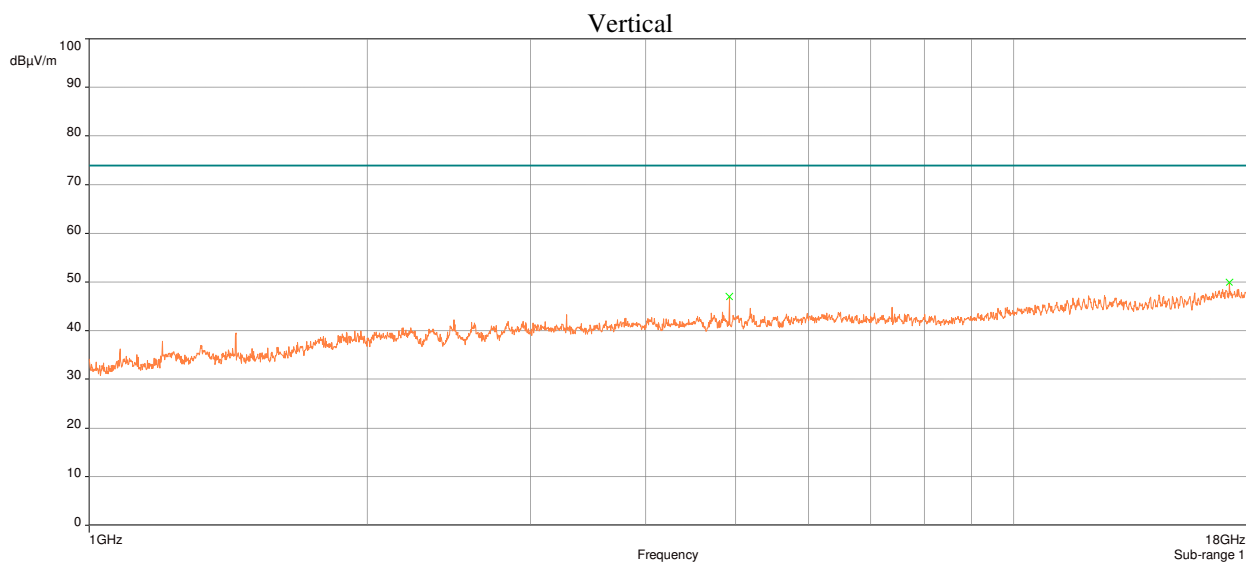
Plot 8: Radiated Spurious Emissions Requirements, 802.11b, High Channel 2462MHz, Peak
