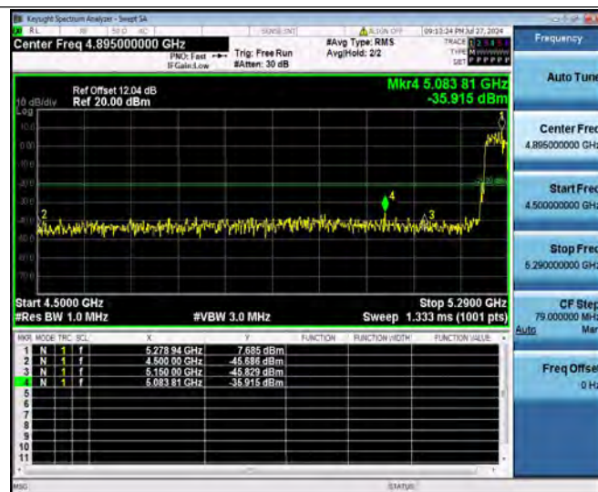
11N40SISO_Ant1_High_5310_Peak
