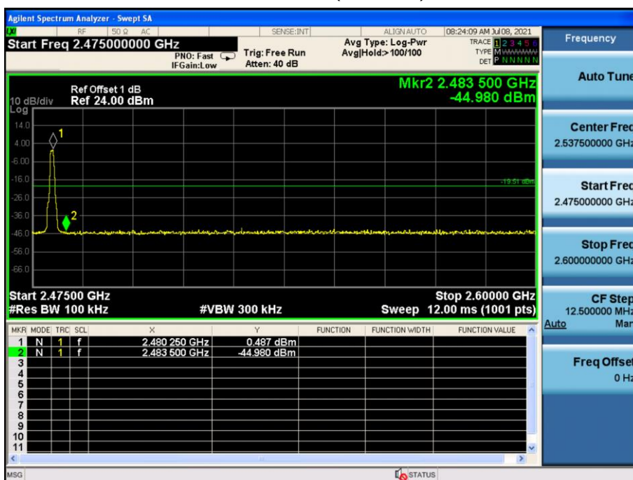
Mode 1 CH39(2480MHz)
