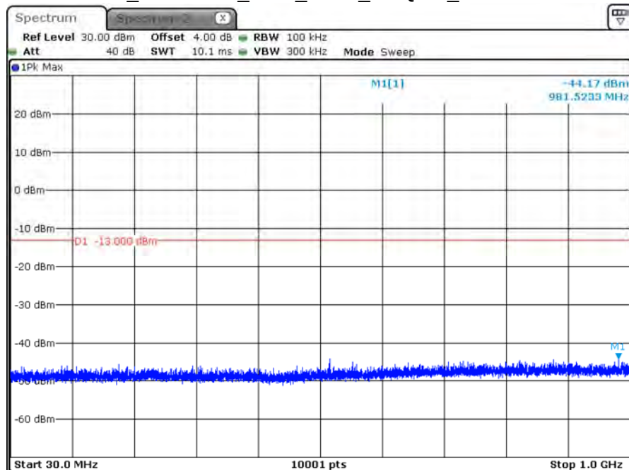
B66_CH132322_1.4M_1RB0_16-QAM_Below 1G
