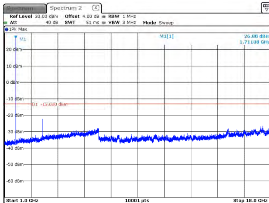
B66_CH131987_3M_1RB0_QPSK_Above 1G
