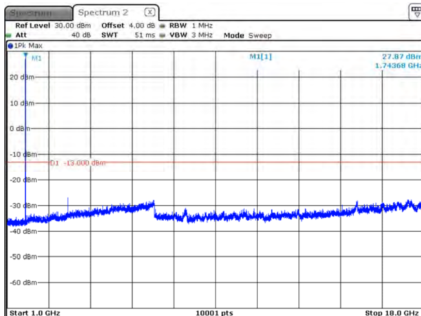
B66_CH132322_5M_1RB0_16-QAM_Above 1G
