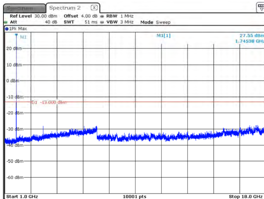
B66_CH132322_1.4M_1RB0_16-QAM_Above 1G
