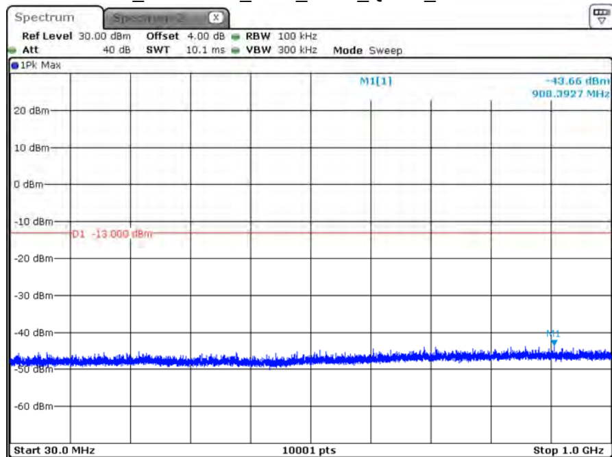
B66_CH132322_1.4M_1RB0_QPSK_Below 1G
