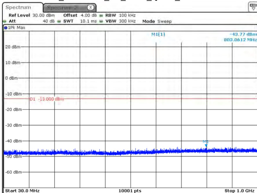
B66_CH131987_3M_1RB0_QPSK_Below 1G
