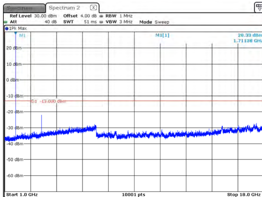
B66_CH131997_5M_1RB0_16-QAM_Above 1G
