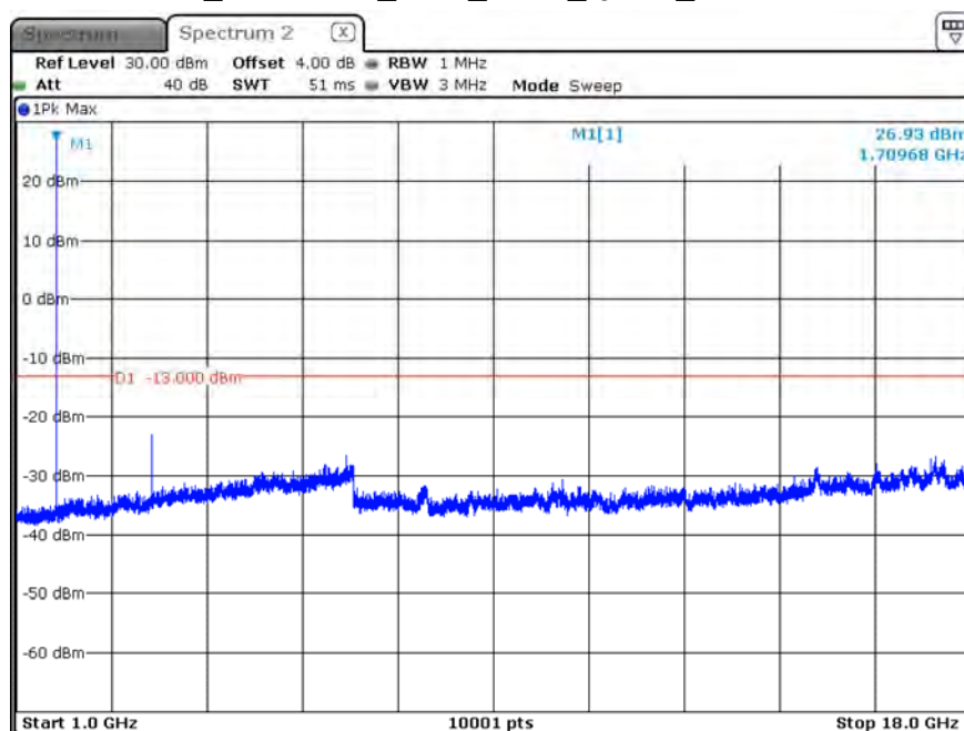
B66_CH131979_1.4M_1RB0_QPSK_Above 1G
