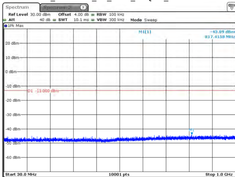
B66_CH131997_5M_1RB0_16-QAM_Below 1G
