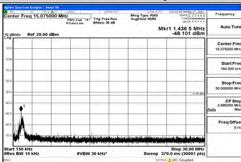
Band66-5MHz-QPSK-131997-1RB#0-Range3:30~1000MHz
