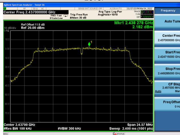
802.11g,2437MHz, Ant1, Plot 1, Reference Level
