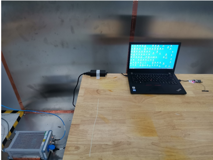
Photograph 3: Set-up for Conducted Emissions ON AC mains
