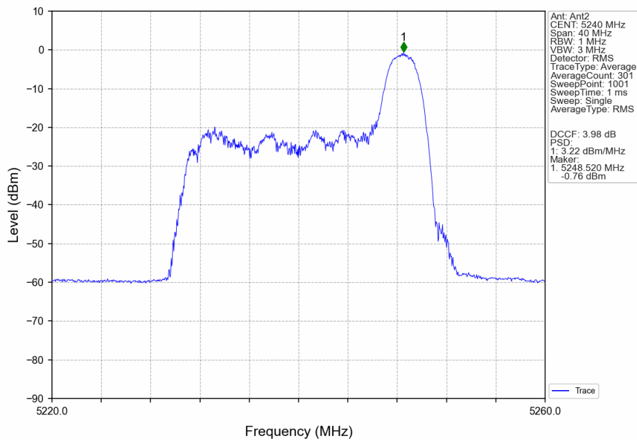
802.11ax(HEW20)_HCH_5240MHz_RU26_Right_Ant2_NTNV
