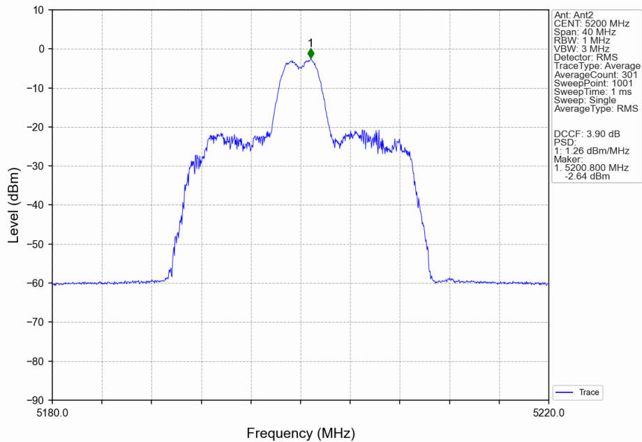
802.11ax(HEW20)_MCH_5200MHz_RU26_Mid_Ant2_NTNV
