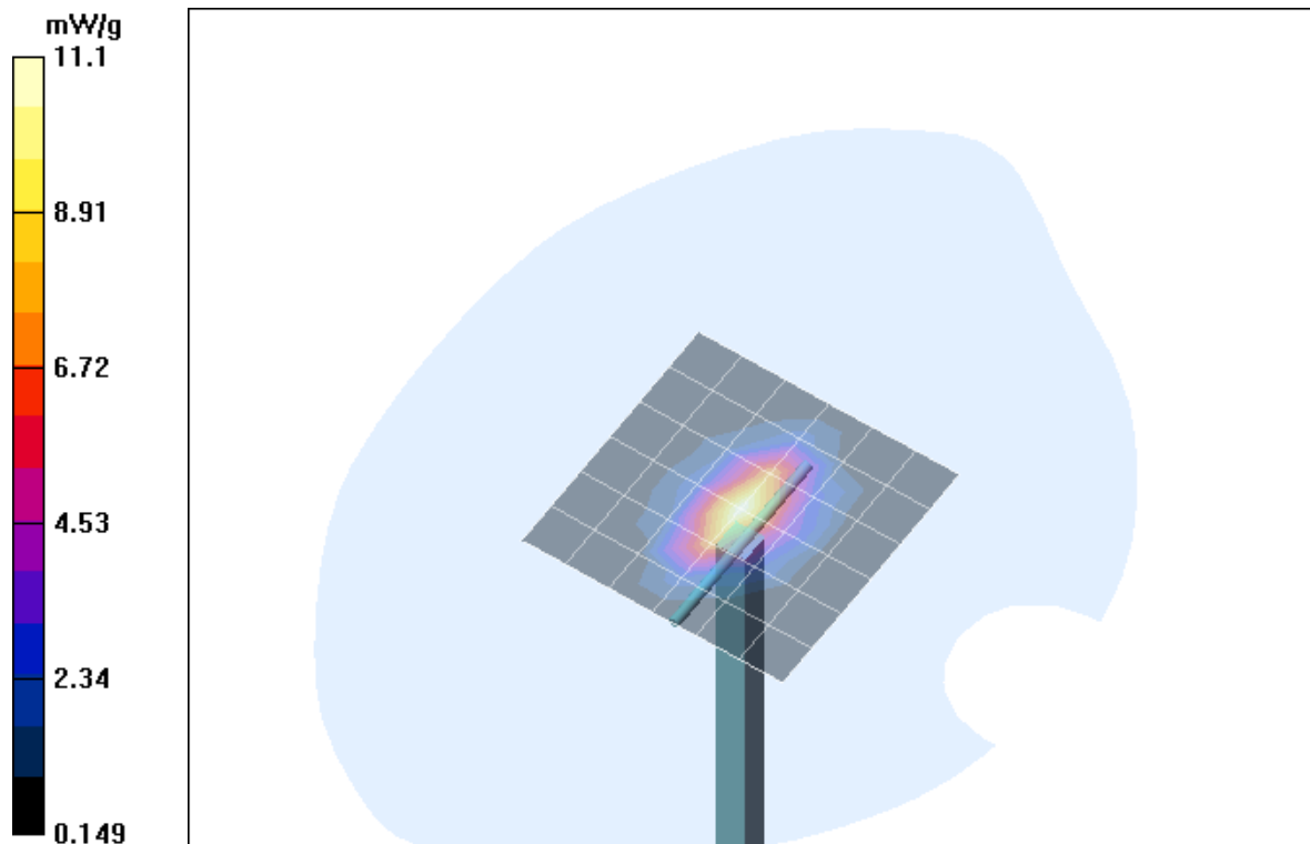
Fig. 11: Validation measurement 1900 MHz body (May 13, 2004), coarse grid. Ambient Temperature: 19.9° C, Liquid Temperature: 19.6° C.
