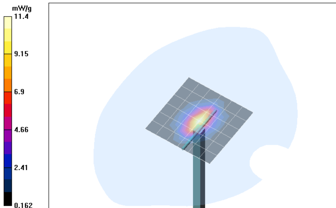
Fig. 10: Validation measurement 1900 MHz Head (April 21, 2004), coarse grid. Ambient Temperature: 22.0° C, Liquid Temperature: 20.6 C.
