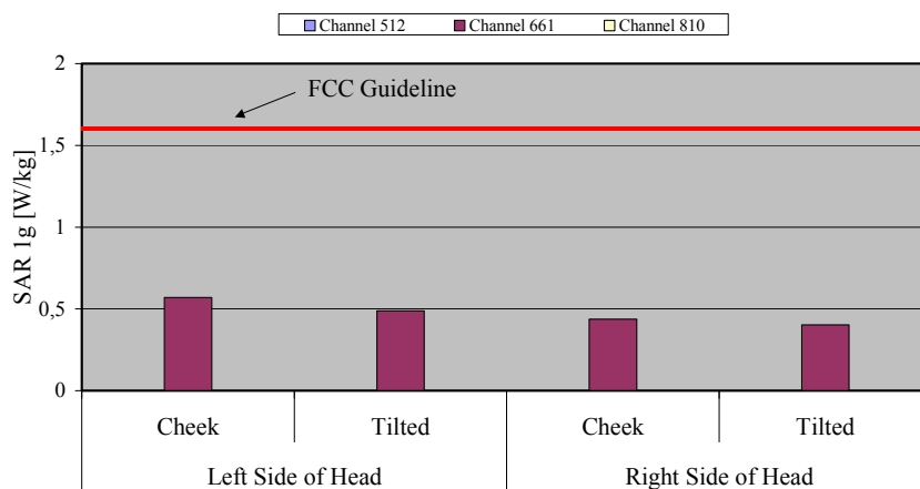
Fig. 8: The measured head phantom SAR values for the Alcatel One Touch 756 for PCS 1900 in comparison to the FCC exposure limit.
