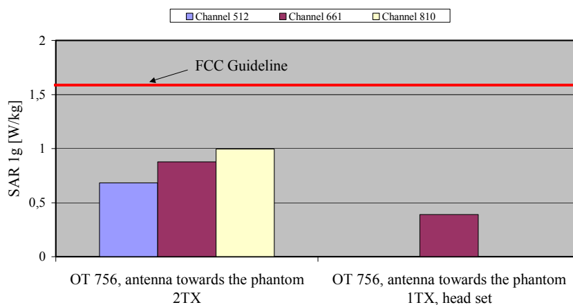
Fig. 9: The measured SAR values in body-worn configuration for the Alcatel One Touch 756 for PCS 1900 (1 TX and 2 TX slots, gap = 2.0 cm) in comparison to the FCC exposure limit.
