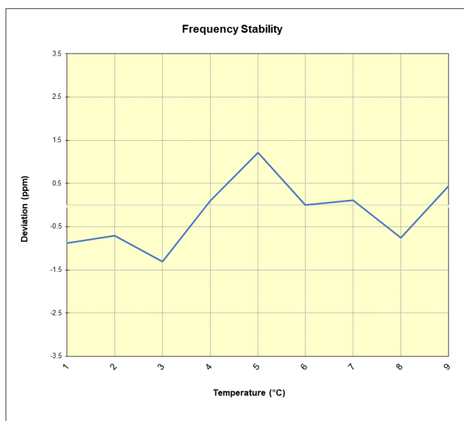
Plot 7-130. LTE Band 66/4 Frequency Stability Chart
