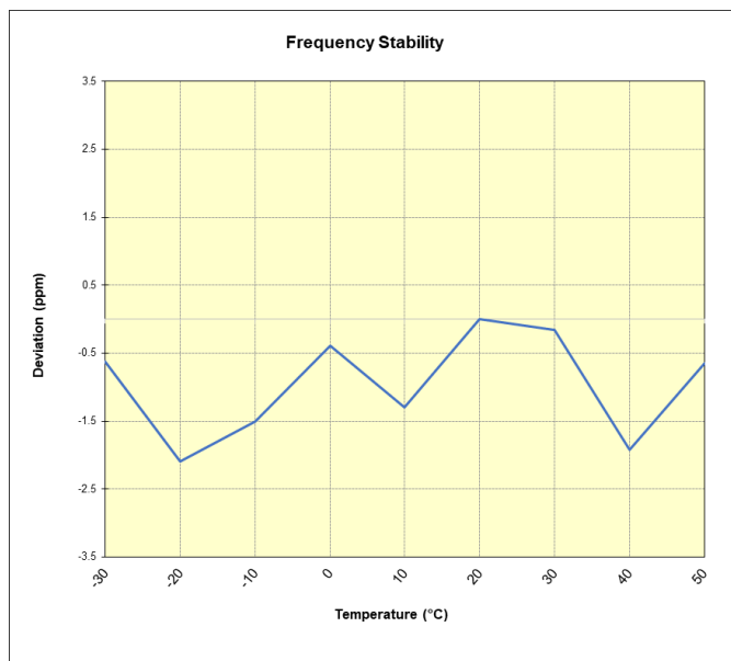
Plot 7-128. LTE Band 12 Frequency Stability Chart
