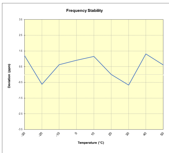
Plot 7-129. LTE Band 13 Frequency Stability Chart
