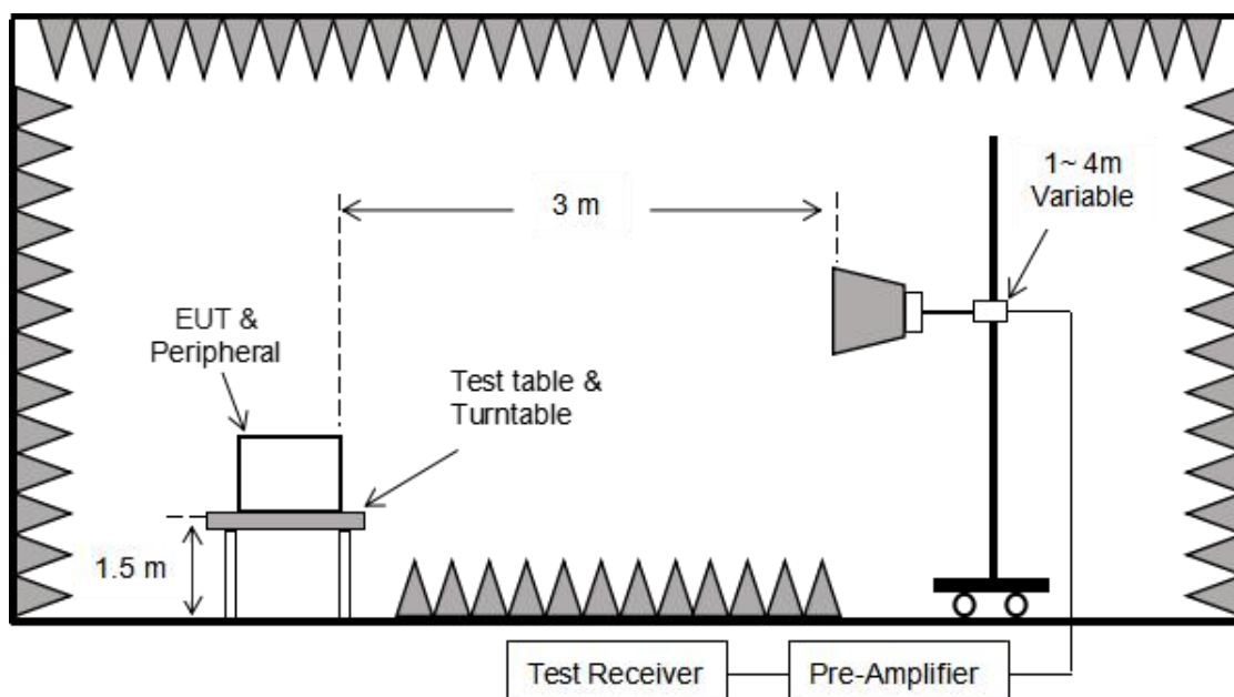
Figure 3. Above 1 GHz
