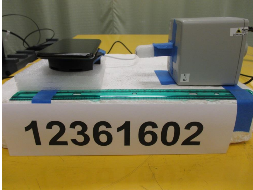
S1, RF EXPOSURE SETUP PHOTO
