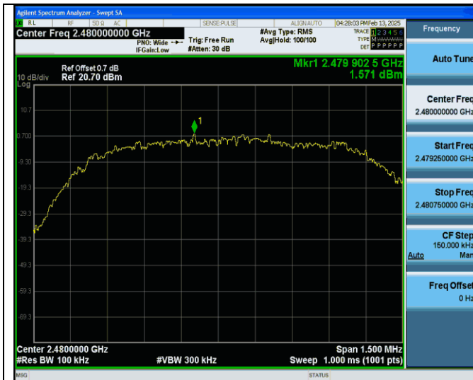
3DH5-Ant1-2480-0~Reference-PASS
