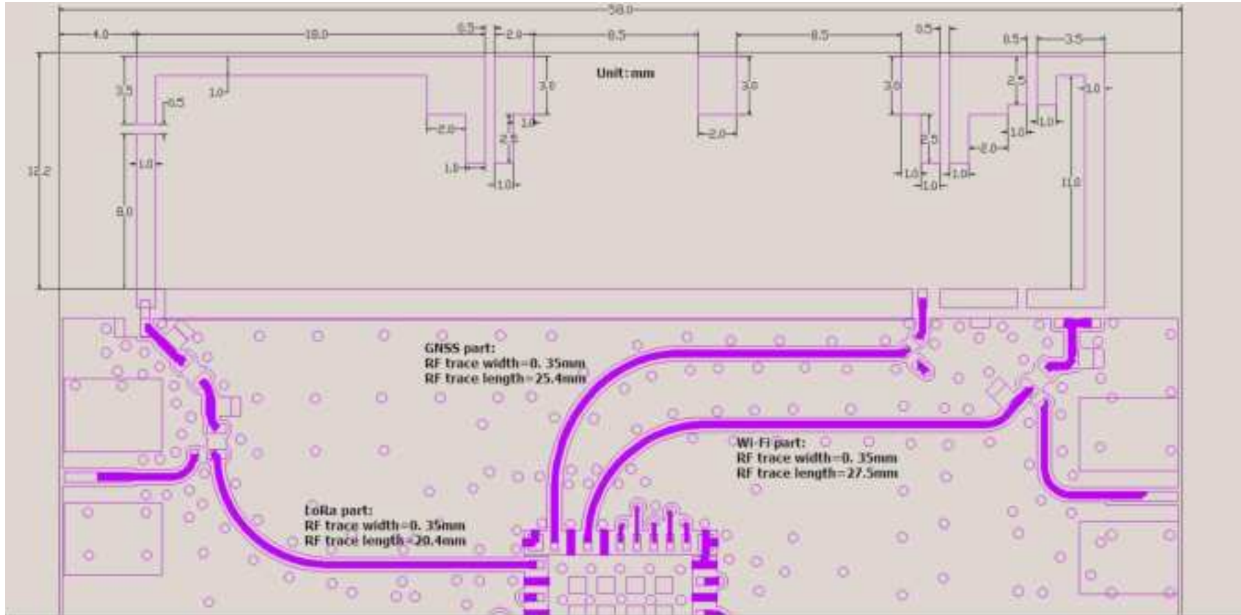
PCB drawing for the antenna
