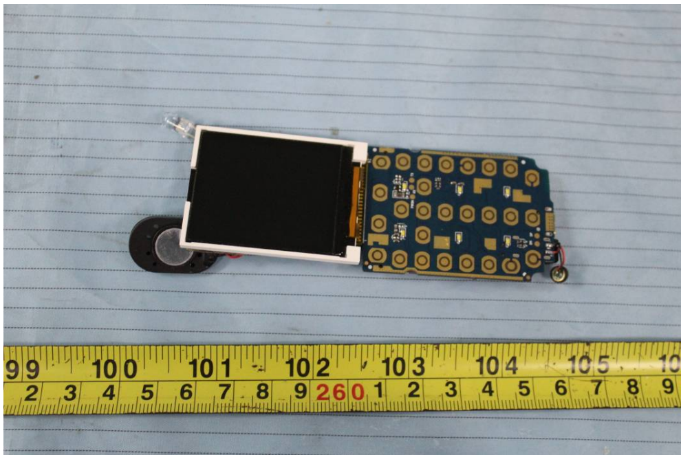
EUT – Main Board Top Shielding off View 1
