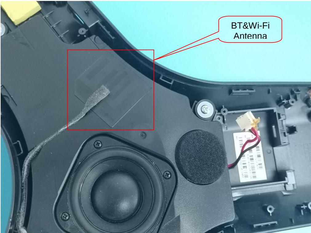
BT&Wi-Fi Antenna
