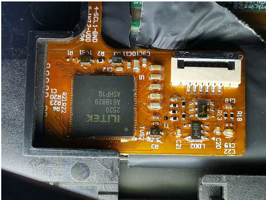
Chip8
