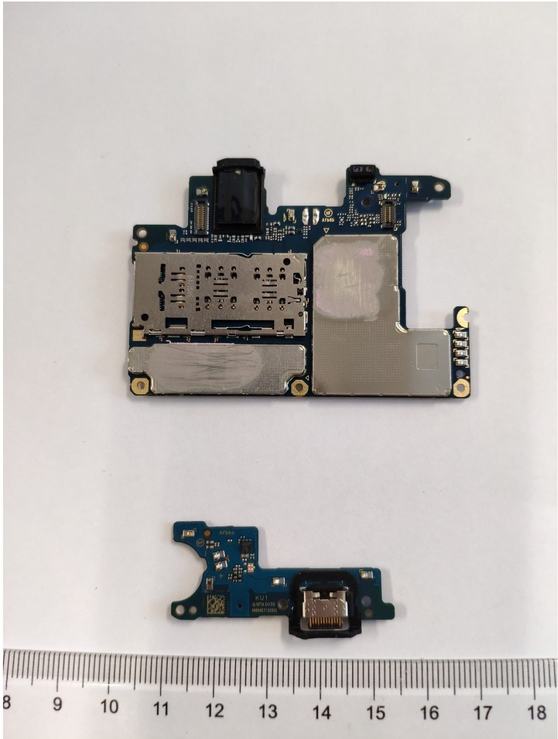
PCB06:
