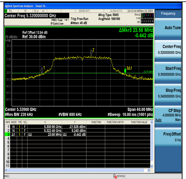
11A-CDD-Ant7-5320
