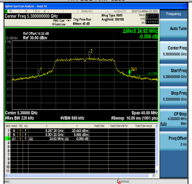
11A-CDD-Ant7-5300
