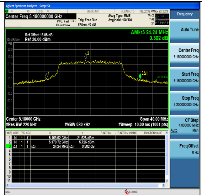
11A-CDD-Ant7-5180
