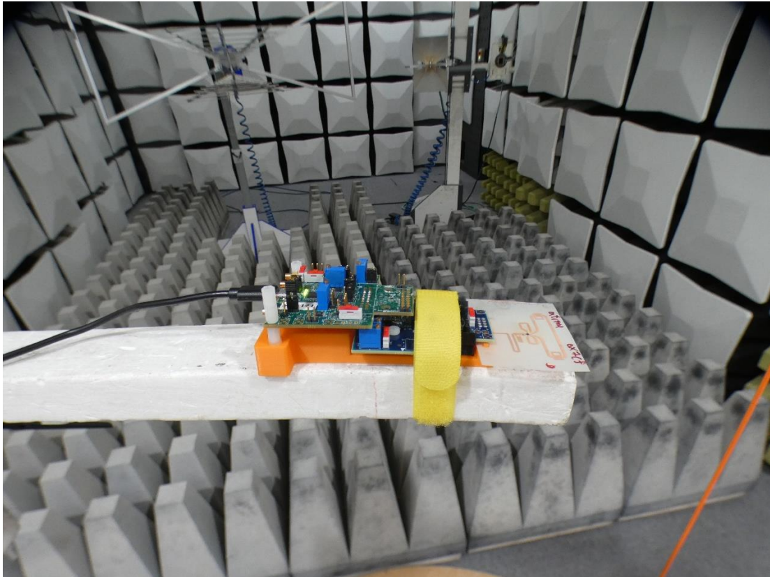
Photo 5: Picture of the EUT
