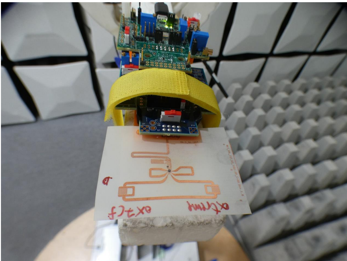
Photo 6: Picture of the EUT
