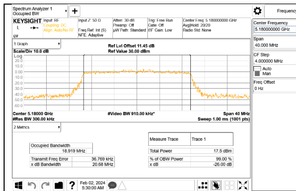
11be EHT20 LOW CHANNEL TX0 99% Bandwidth
