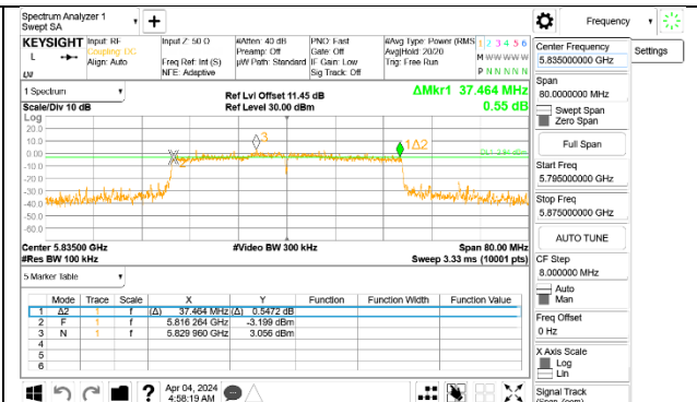
11be EHT40 LOW CHANNEL TX0 6dB Bandwidth
