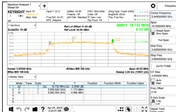
11be EHT20 LOW CHANNEL TX0 6dB Bandwidth
