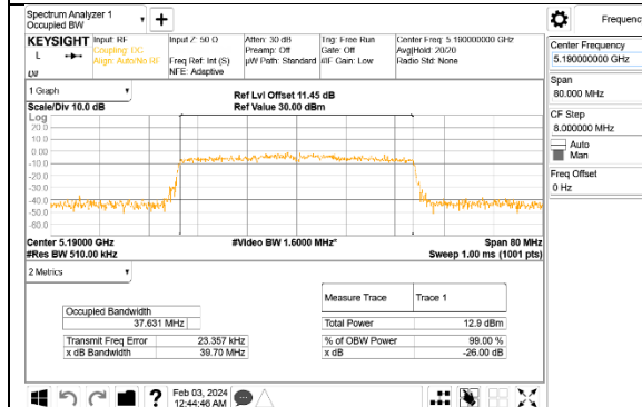
11be EHT40 LOW CHANNEL TX0 99% Bandwidth
