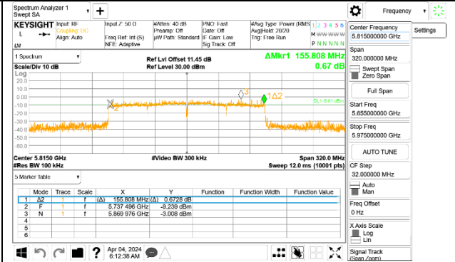
11be EHT160 MID CHANNEL TX0 6dB Bandwidth
