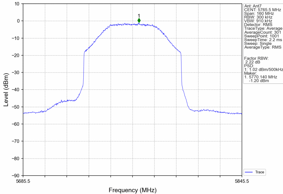
80M_LCH_5765.5MHz_MIMO_NTNV
