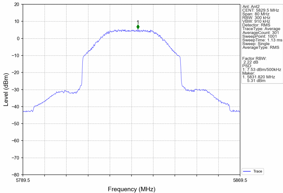
40M_HCH_5829.5MHz_Ant2_NTNV
