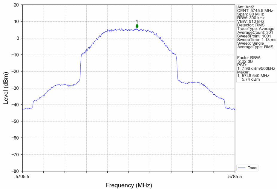
40M_LCH_5745.5MHz_Ant2_NTNV
