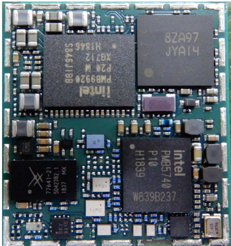
Internal View of EUT – 4
