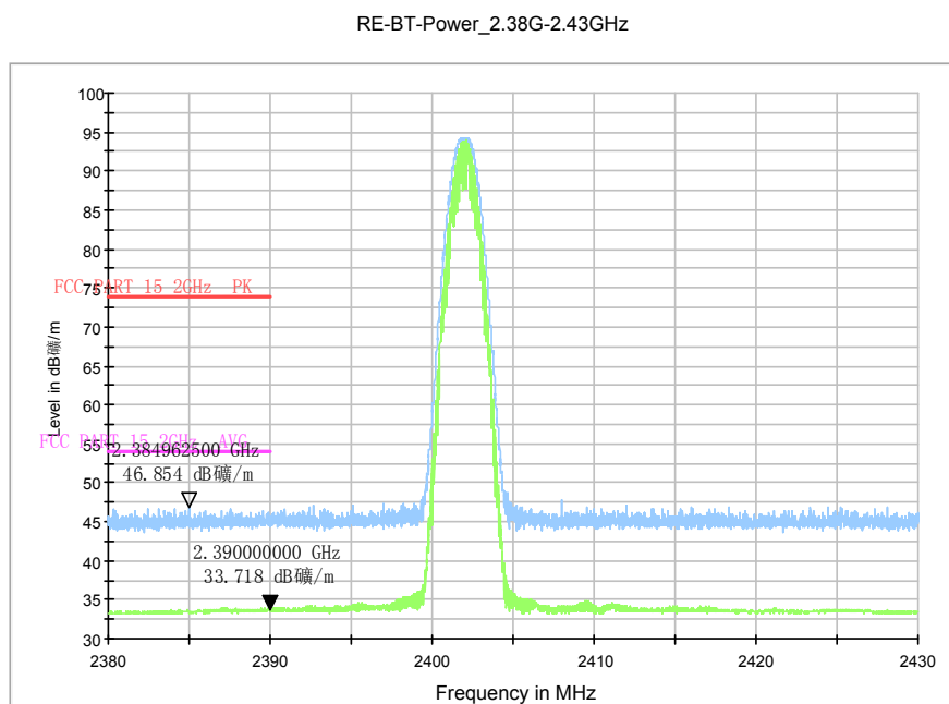
Fig.65. Radiated emission (Power): GFSK, low channel
