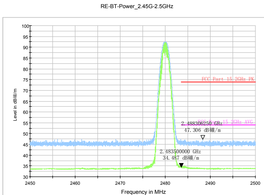
Fig.66. Radiated emission (Power) GFSK, high channel
