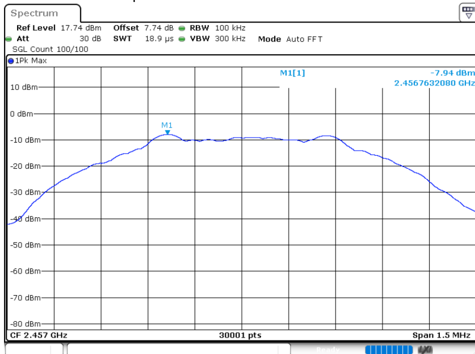
Tx. Spurious NVNT ANT+ 2457MHz Ant1 Ref
