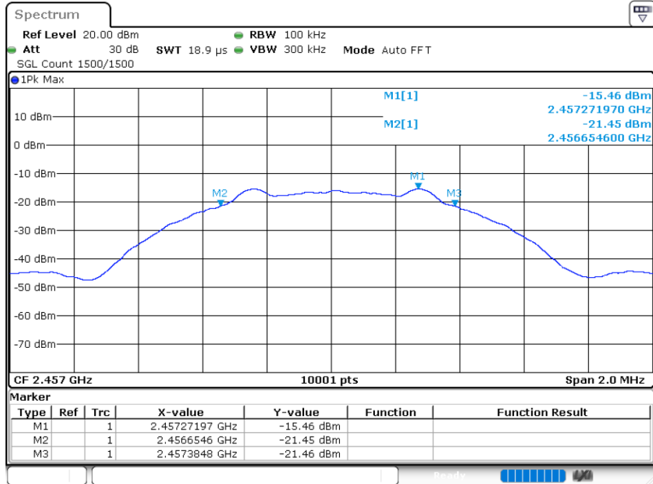
-6 dB BW NVNT ANT+ 2457MHz Ant1
