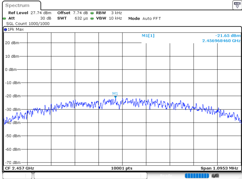
PSD NVNT ANT+ 2457MHz Ant1
