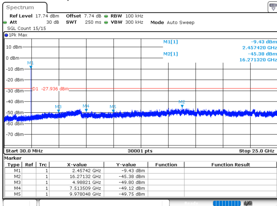
Tx. Spurious NVNT ANT+ 2457MHz Ant1 Emission
