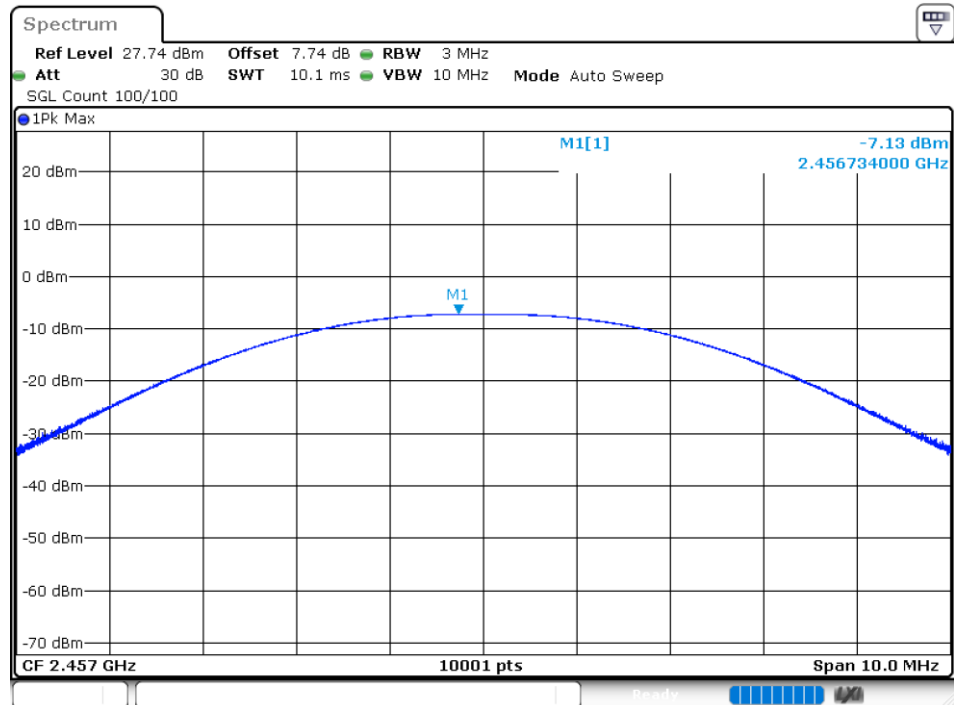
Power NVNT ANT+ 2457MHz Ant1
