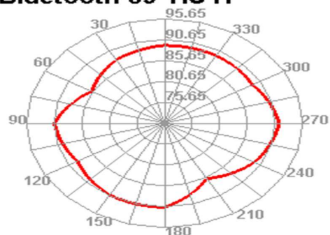
Bluetooth 39 TIS H
