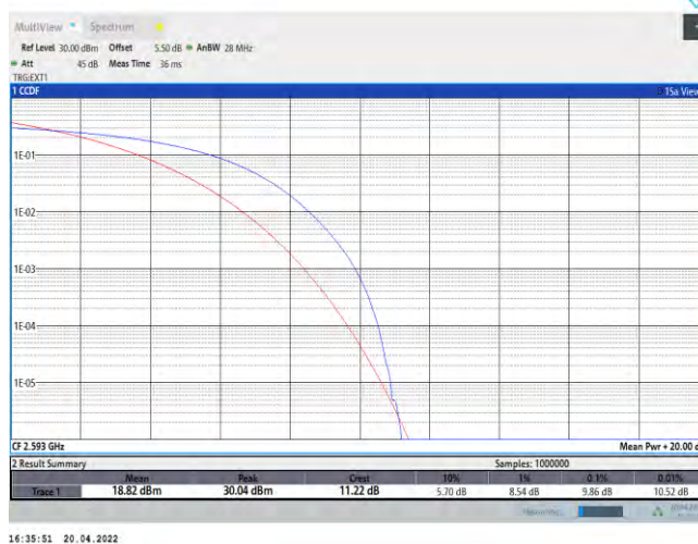
41-41-20MHz-20MHz-QPSK-QPSK-40521-40719-100RB#0-100RB#0
