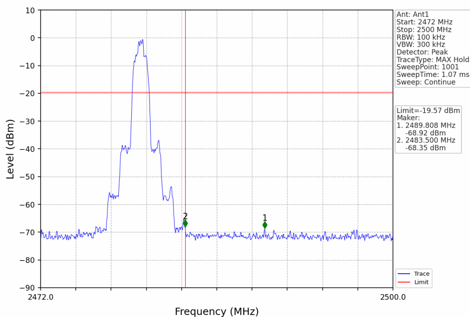
8DPSK_3DH5_HCH_2480MHz_Ant1_NTNV
