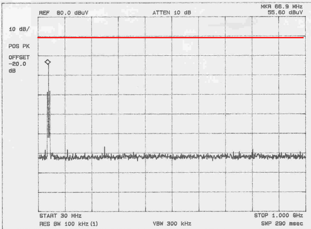
CH4 Record
