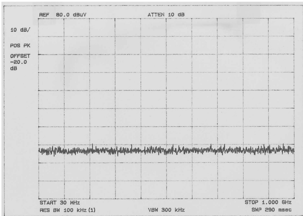
CH4 Record
