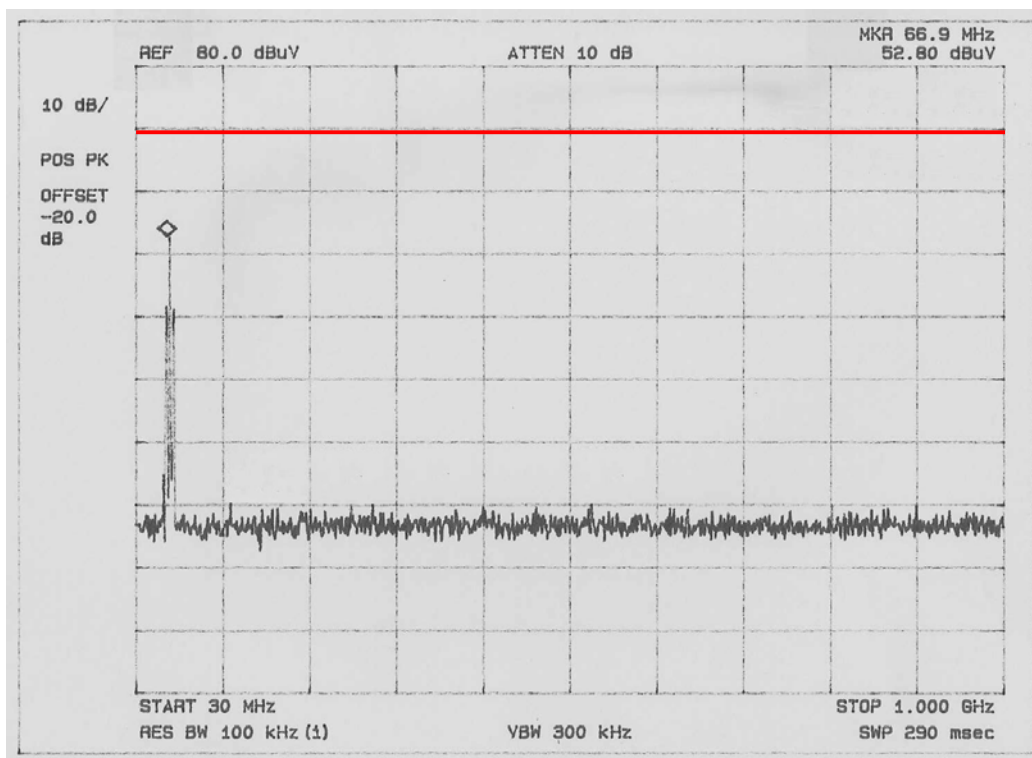
CH4 Playback
