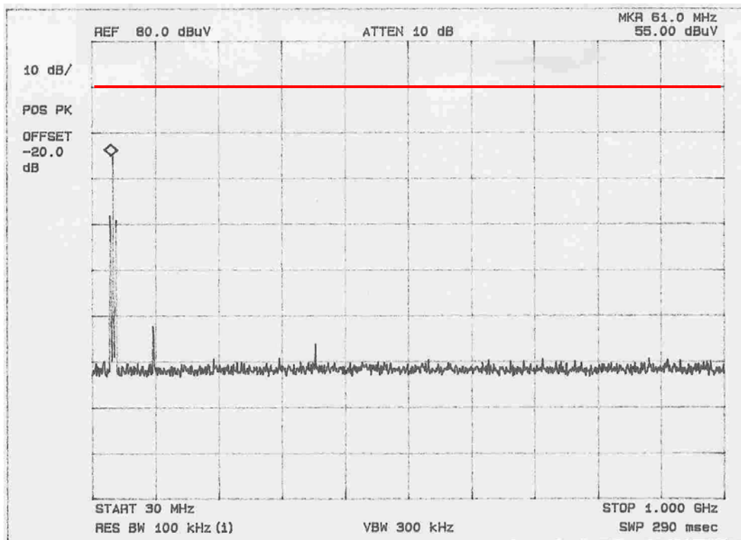
CH3 Playback
