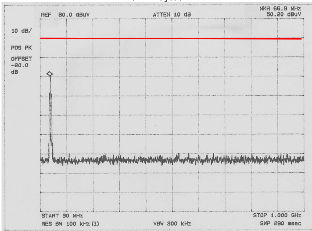
CH4 Record
