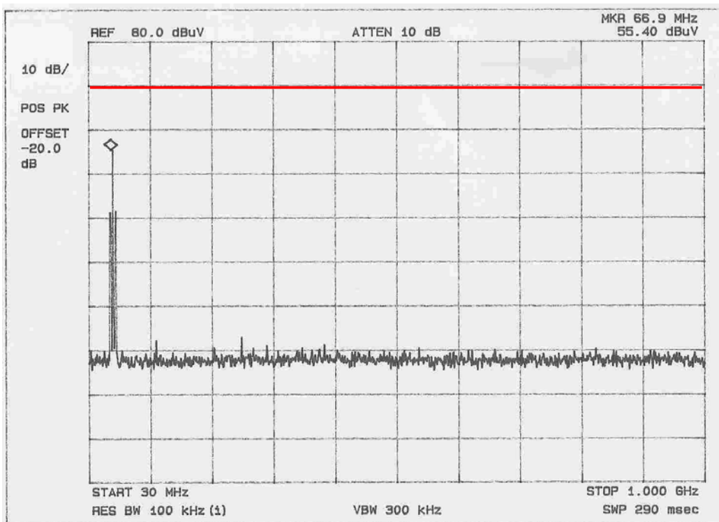
CH4 Playback
