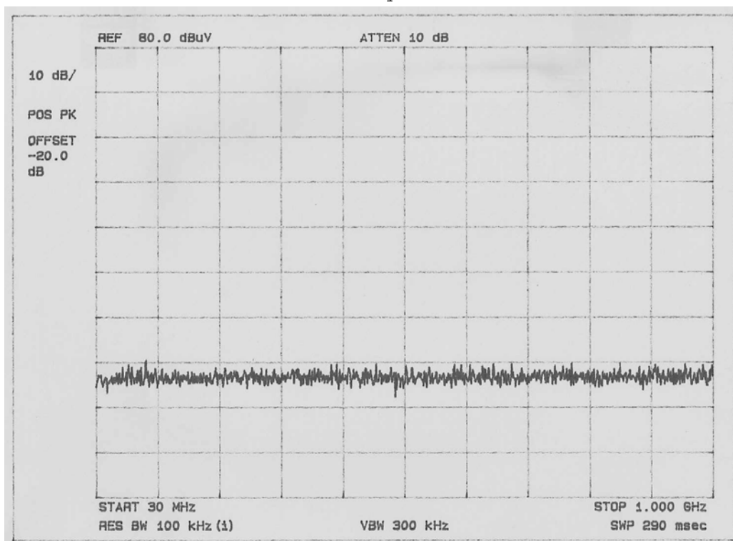
CH3 Record
