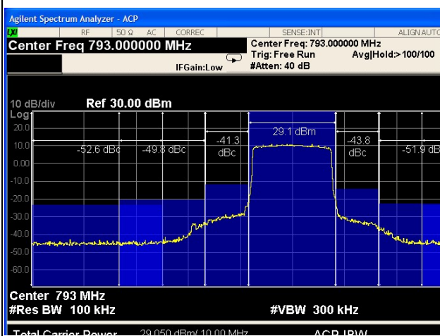
LTE Band 14 QPSK 100%RB 10MHz CH Middle
