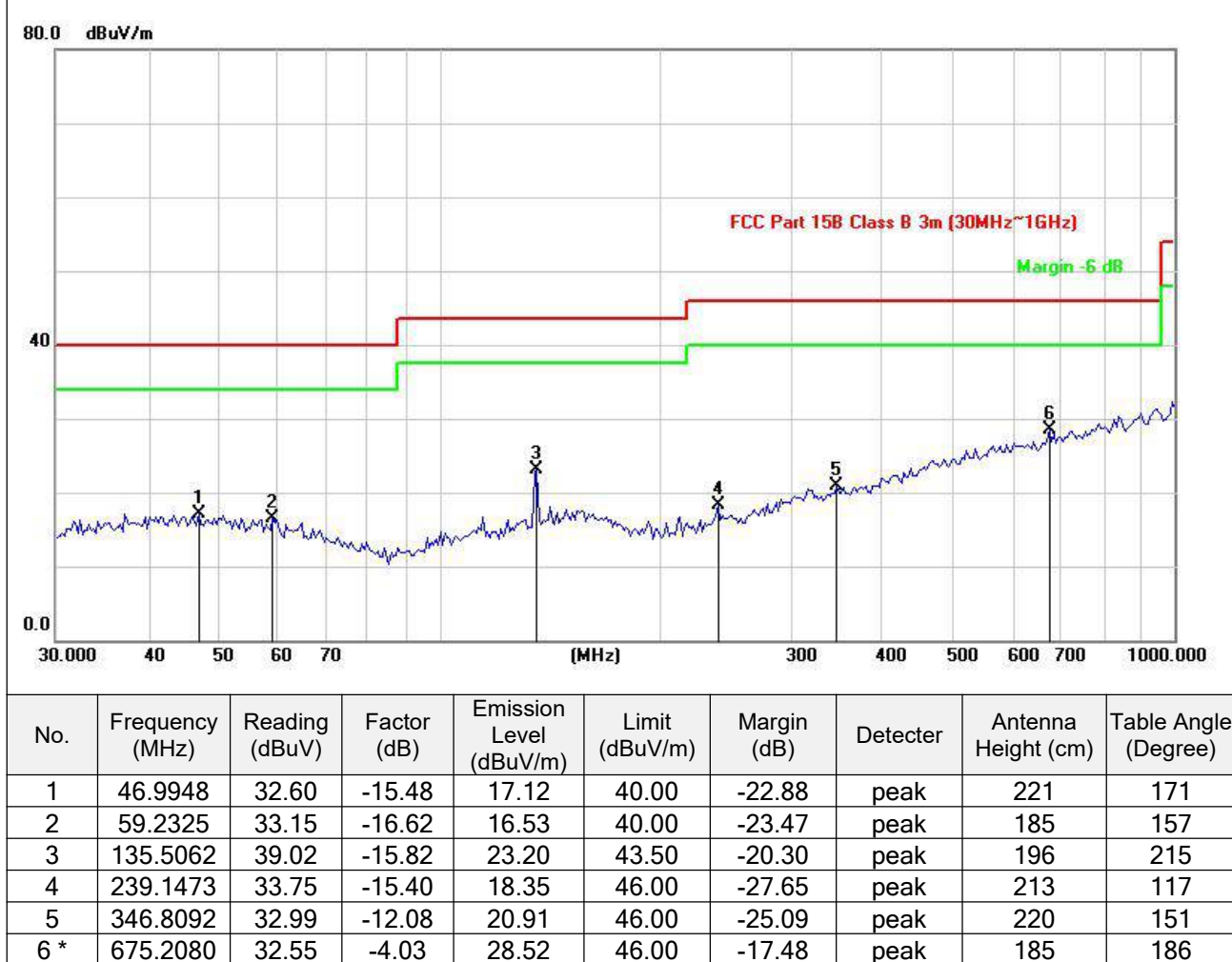
Antenna Polarity & Test Distance: Horizontal at 3 m
