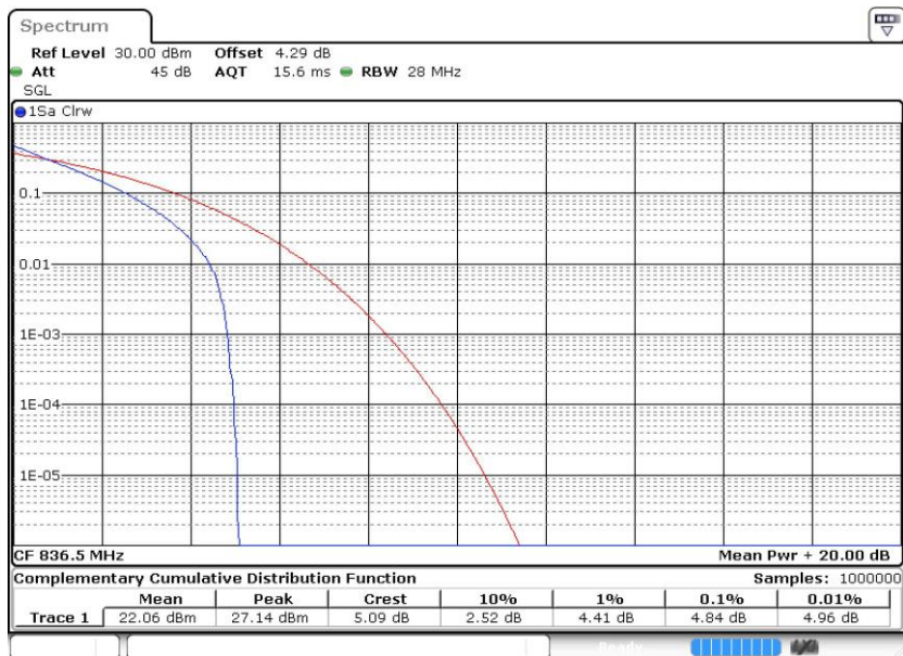
Band5-10MHz-QPSK-20525-50RB#0
