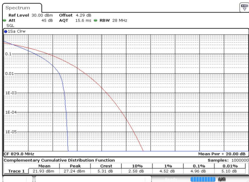
Band5-10MHz-QPSK-20450-50RB#0
