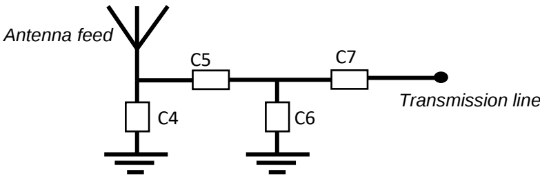
Matching circuit
