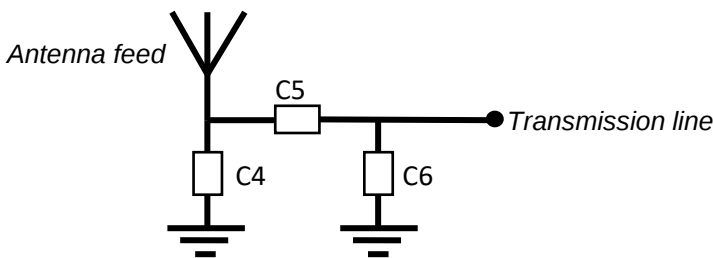
Matching circuit
