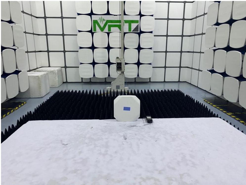
Description: Radiated Emission Test Setup for Above 1GHz Test Mode 3
