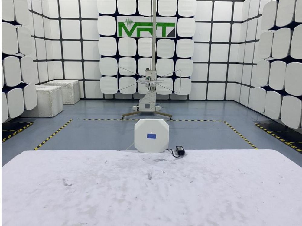
Description: Radiated Emission Test Setup for Below 1GHz Test Mode 3
