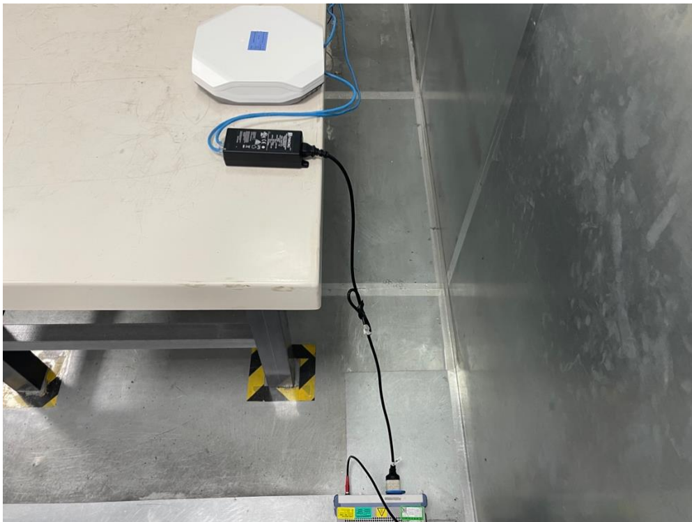
Description: Back View of Conducted Emission Test Setup for Power Port Test Mode 2
