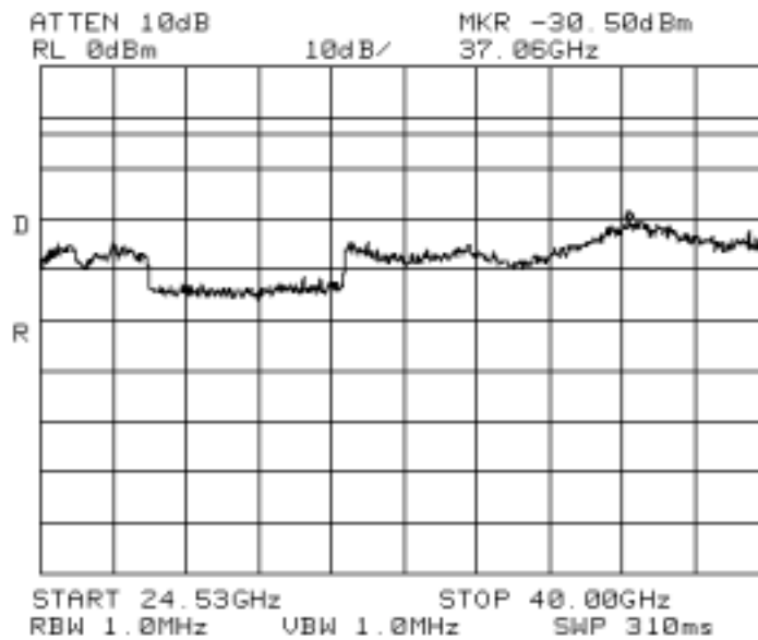
Fig. A-9 (Conducted Spurious Emissions, 1 carrier, 24.53 – 40GHz)
