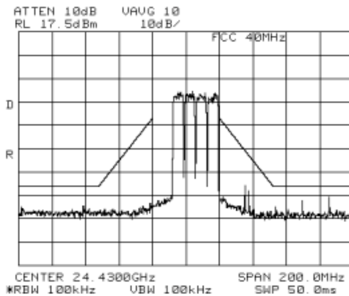
Fig. A-6 (Spectrum Mask, channel T, 4 carriers)
