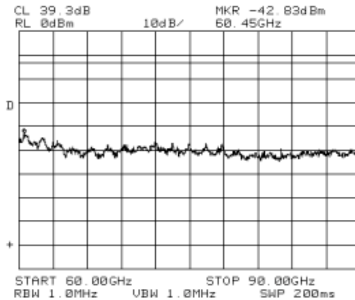
Fig. A-17 (Conducted Spurious Emissions, 4 carriers, 60 – 90GHz)
