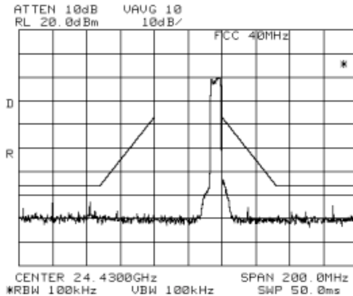
Fig. A-4 (Spectrum Mask, channel T, 1 carrier)
