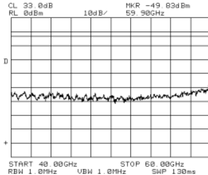
Fig. A-16 (Conducted Spurious Emissions, 4 carriers, 40 – 60GHz)
