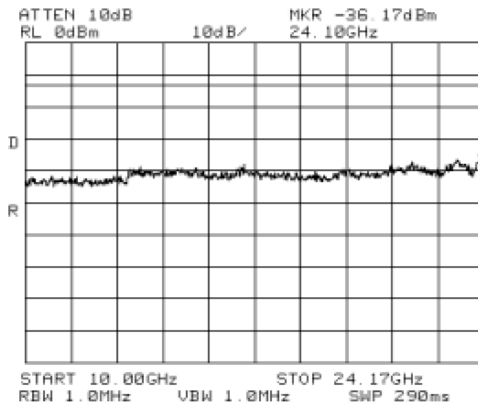
Fig. A-14 (Conducted Spurious Emissions, 4 carriers, 10 – 24.17GHz)
