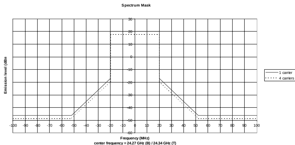
Fig. 5-1: Spectrum Mask limit
