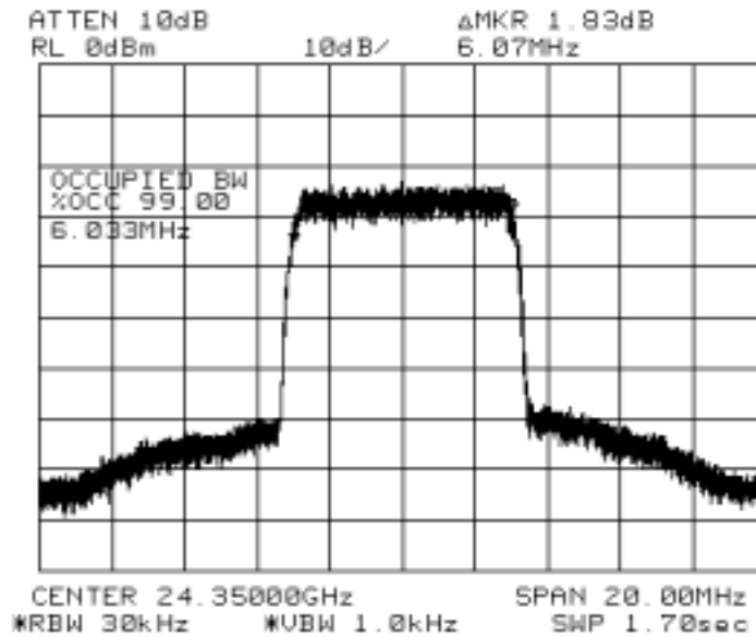
Fig. A-1 (99% Occupied Bandwidth, 1 carrier)
