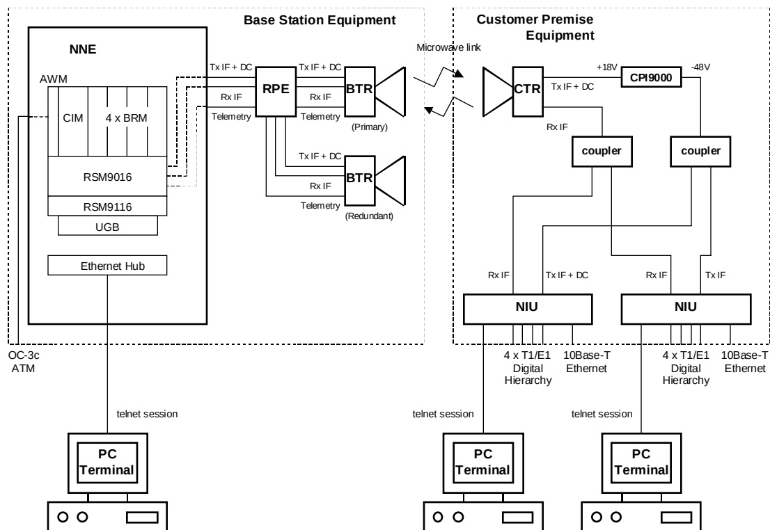
Fig. 3-1: Nortel Networks iBWA System 5100 TDMA
