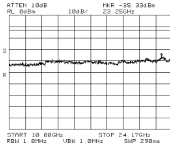
Fig. A-8 (Conducted Spurious Emissions, 1 carrier, 10 – 24.17GHz)
