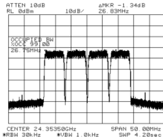
Fig. A-2 (99% Occupied Bandwidth, 4 carriers)
