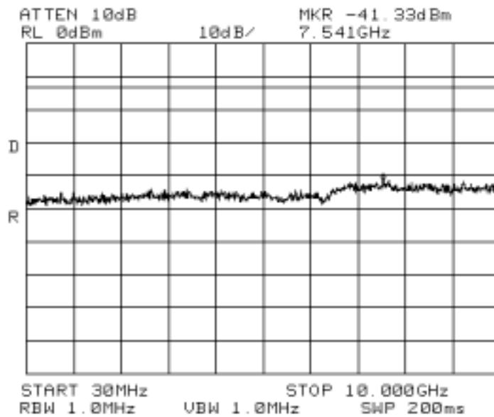
Fig. A-7 (Conducted Spurious Emissions, 1 carrier, 30MHz – 10GHz)
