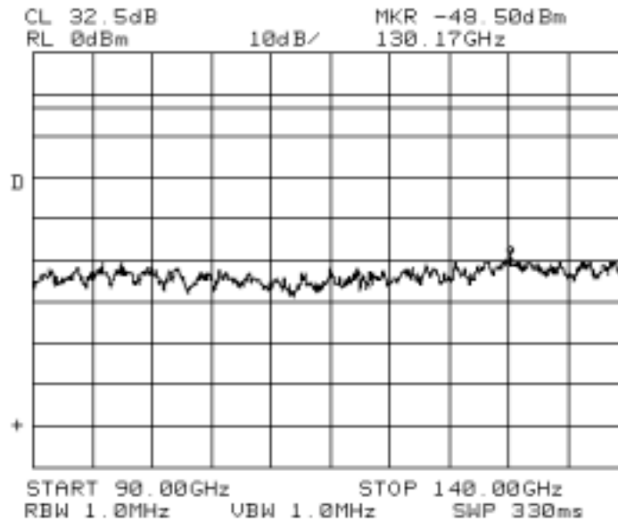
Fig. A-18 (Conducted Spurious Emissions, 4 carriers, 90 – 140GHz)
