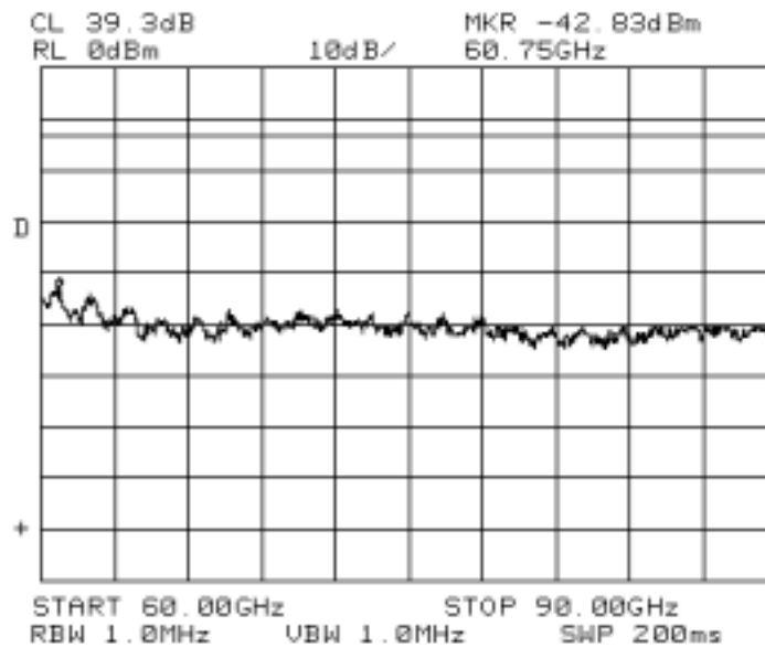
Fig. A-11 (Conducted Spurious Emissions, 1 carrier, 60 – 90GHz)
