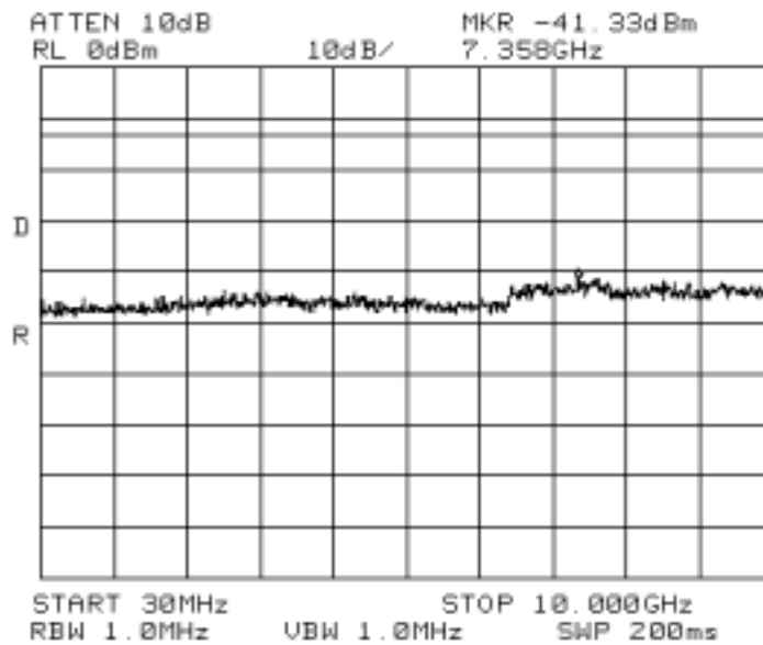
Fig. A-13 (Conducted Spurious Emissions, 4 carriers, 30MHz – 10GHz)
