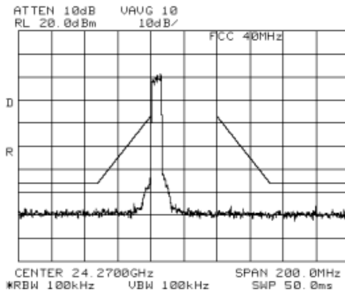
Fig. A-3 (Spectrum Mask, channel B, 1 carrier)
