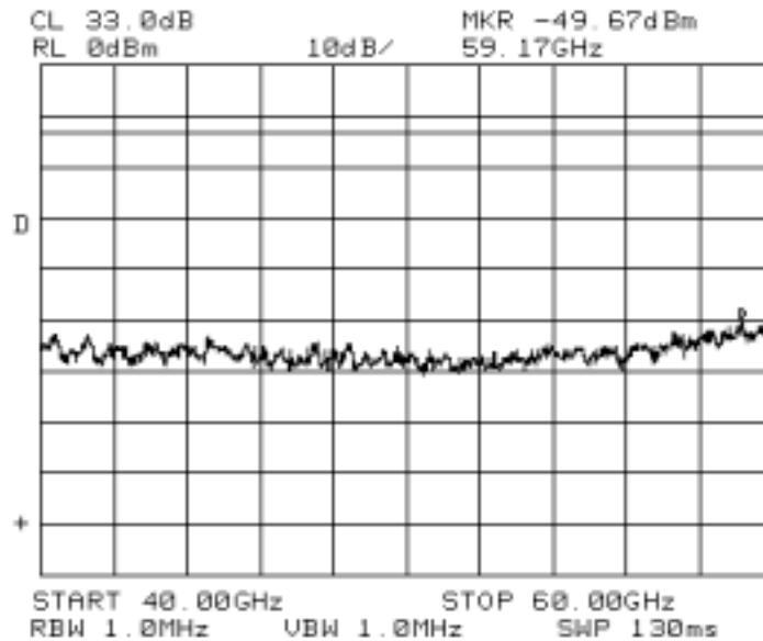
Fig. A-10 (Conducted Spurious Emissions, 1 carrier, 40 – 60GHz)
