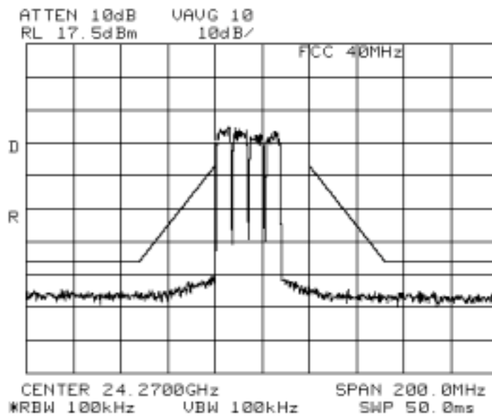
Fig. A-5 (Spectrum Mask, channel B, 4 carriers)
