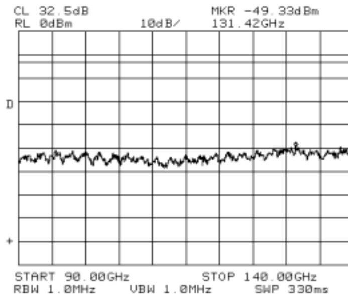
Fig. A-12 (Conducted Spurious Emissions, 1 carrier, 90 – 140GHz)
