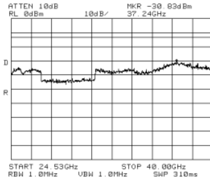
Fig. A-15 (Conducted Spurious Emissions, 4 carriers, 24.53 – 40GHz)
