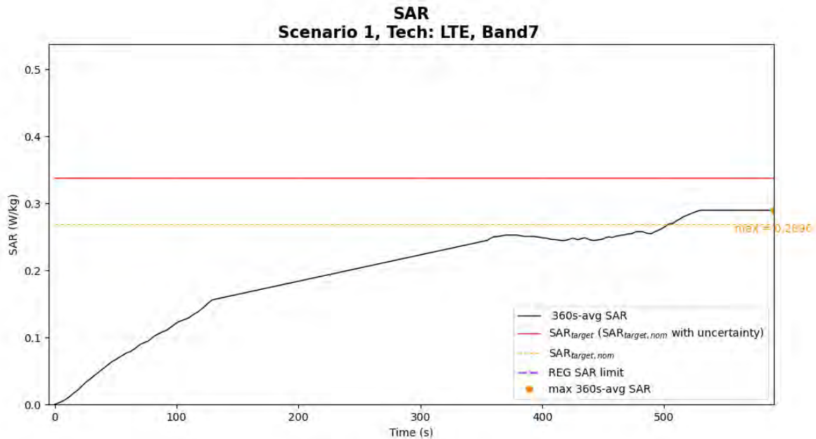
Figure 5-26 Time-averaged SAR for case 13 (LTE B7)
