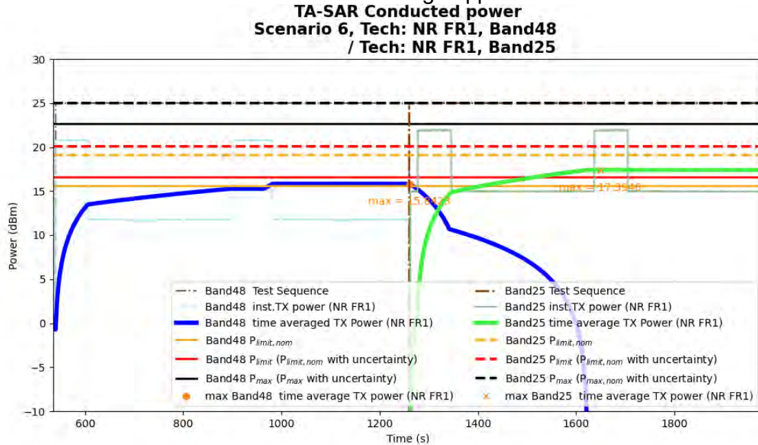
Figure 5-57 Time-averaged conducted TX power over time for case 23 (sub6 NR B48 and B25)
