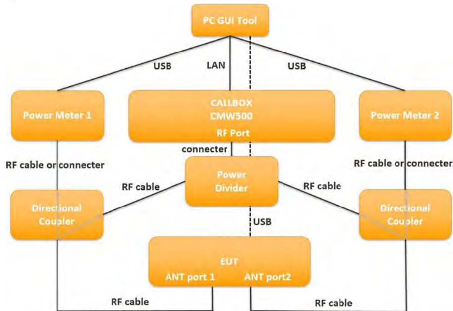
Figure 5-3 TA-SAR conductive power test setup block diagram for scenarios 2/4/6
