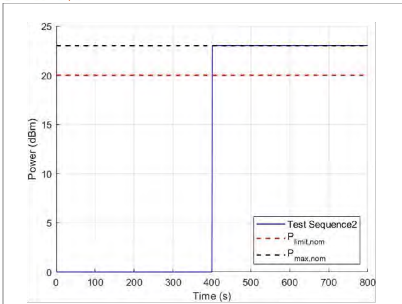
Figure 4-3 Test sequence 2
