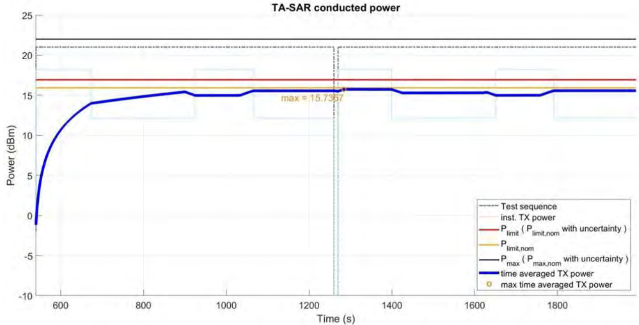
Figure 5-67 Time-averaged conducted TX power over time for case 24 (sub6 NR B25)
