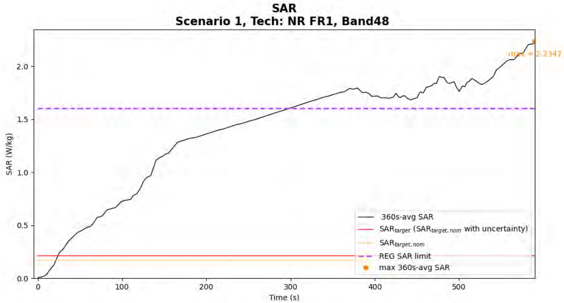
Figure 5-16 Time-averaged SAR for case 17 (sub6 NR n48)
