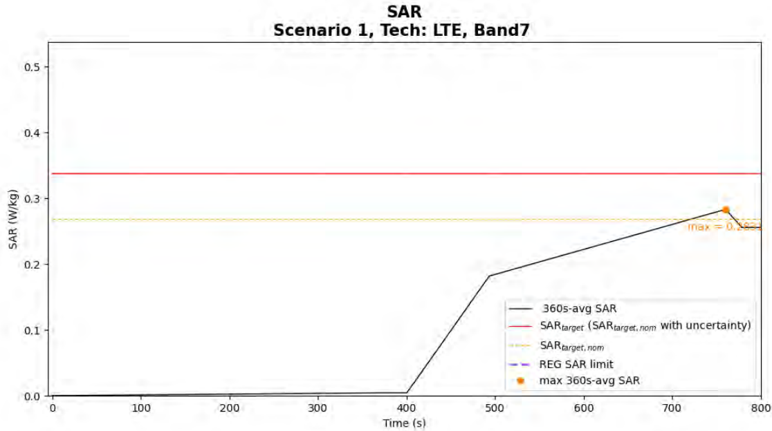
Figure 5-22 Time-averaged SAR for case 7 (LTE B7)
