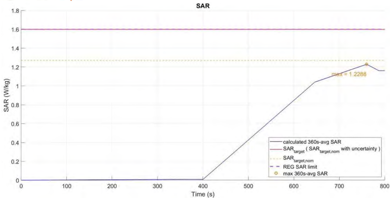
Figure 5-32 Time-averaged SAR for case 6 (WCDMA B2)
