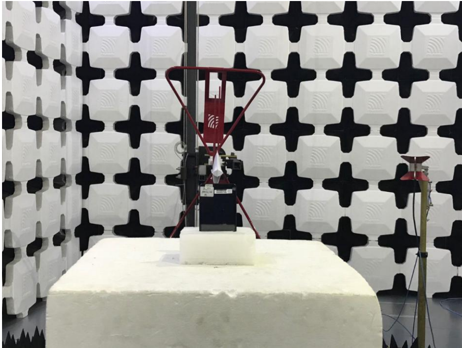
3. Radiated Emissions (Part 15C) (1-18GHz)
