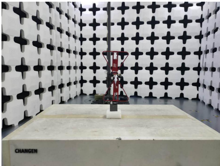
2. Radiated Emissions (Part 15C) (30MHz-1GHz)
